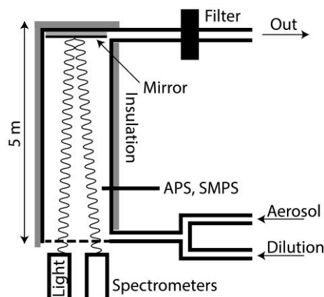
Figure 1. Experimental set-up
