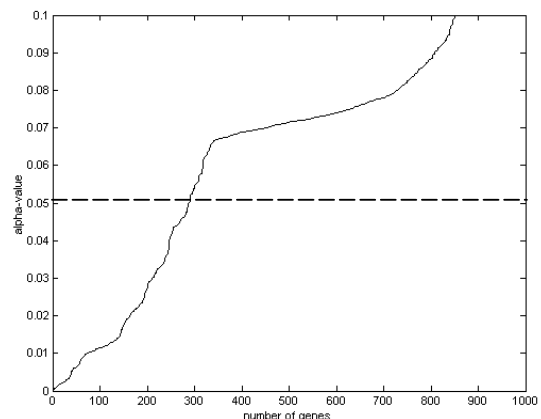
Figure 2. Sorted \alpha -values ( \alpha < 0.1 ).
