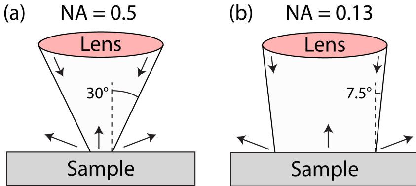
Figure 6. Schematic of the numerical aperture dependence on the shape of the illumination and collection cone for (a) NA = 0.5 and (b) NA = 0.13. With NA = 0.5 the half-angle of the cone is 30° whereas it is 7.5° for NA = 0.13.
