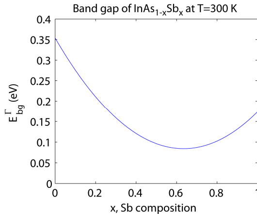
Figure 23. Energy of the fundamental band gap of \text{InAs}_{1-x}\text{Sb}_x at the \Gamma point for the temperature T = 300 K [8].
