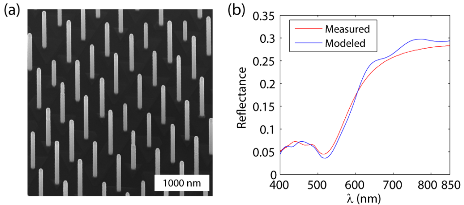
Figure 21. (a) SEM image at 20^\circ tilt from top view of a ZB InAs NW array with p = 500 nm and NWs of D = 73.0 \pm 4.3 nm and L = 1940 \pm 270 nm (see [Paper VIII] for details of the NW growth). (b) Measured reflectance spectrum (red line) of the NW array in (a). For this array the optical metrology method [Paper IX] was applied to determine the NW diameter and length: The best-fit spectrum from modeling (blue line) was obtained for D = 76 nm and L = 1830 nm. Thus, these optically determined dimensions are in very good agreement with the dimensions determined with SEM.
