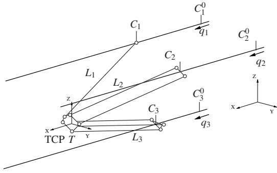
Fig. 2. Gantry-Tau schema with notation for variables and parameters
