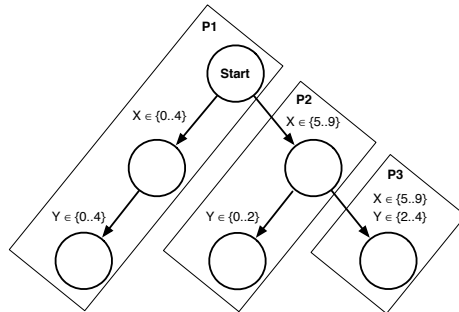
Fig. 2. Parallel search in constraint programming.
