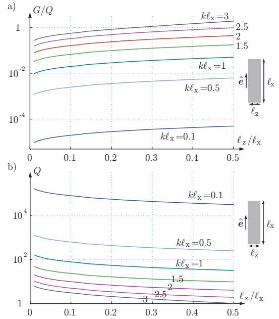
Fig. 1. Upper bounds on G/Q and Q for antennas confined to planar rectangles for k\ell_x = \{0.1, 1, 1.5, 2, 2.5, 3\} .
