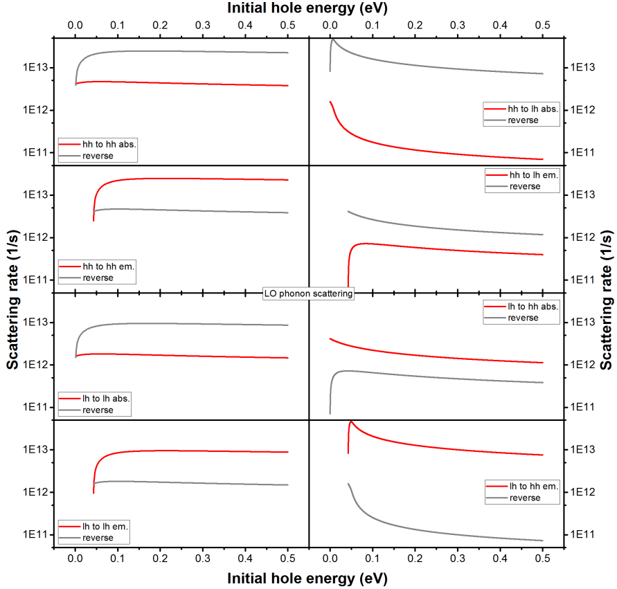
Figure 2.7: Energy dependence of the InP hole scattering rates with LO phonons (absorption and emission) for heavy holes and light holes (red spectra) at 300 K and rates of the respective reverse scattering processes, back to initial hole band, energy, and momentum (grey spectra).
