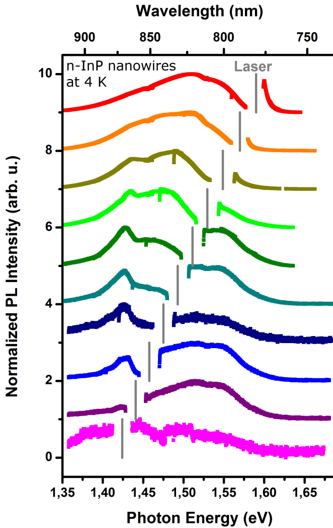
Figure 4.9: Normalized PL spectra for a highly n-doped nanowire sample (corresponding to spectrum III in Fig. 4.4) for different energies of the exciting laser. The gray vertical lines indicate the exciting laser energy. The integration time above the laser energy was 20 times higher than below the laser energy. The cryostat temperature was 4 K.
