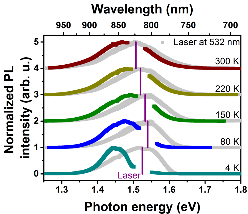
Figure 4.11: Temperature dependence of n-doped InP nanowire PL spectra for 2.33 eV excitation (gray spectra) and excitation at the PL peak maximum (colored spectra). The laser photon energy is indicated by the vertical purple lines.
