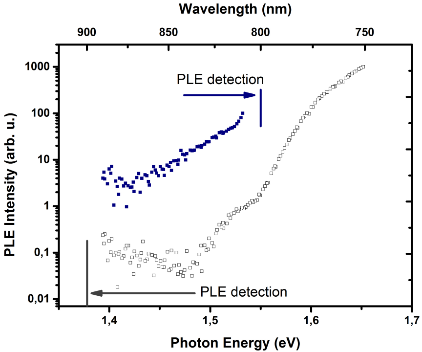
Figure 4.14: 4 K PLE spectra of n-doped InP nanowires (sample IV in Fig. 4.4) with PLE detection below and above the exciting laser, respectively.
