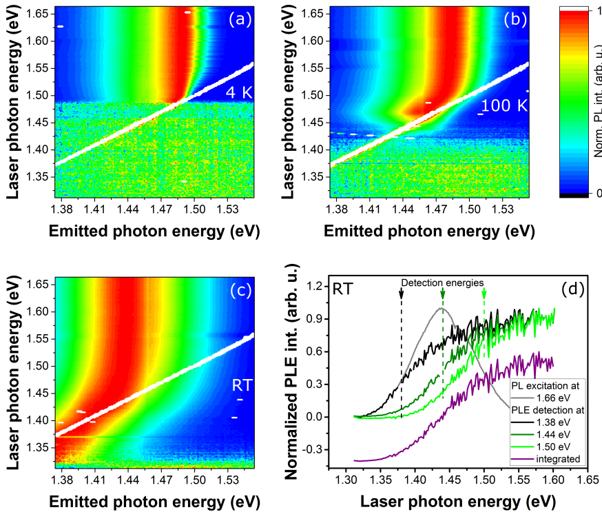
Figure 4.13: Excitation energy dependence of the normalized luminescence of n-doped InP bulk samples as photon energy contour plots measured at 4 K (a), 100 K (b) and at room temperature (c). (d) Normalized room temperature PLE spectra for selected detection energies and integrated PLE intensity. The detection energy is indicated by arrows and vertical dashed lines. The gray spectrum shows the room temperature PL spectrum for 1.66 eV excitation for comparison.
