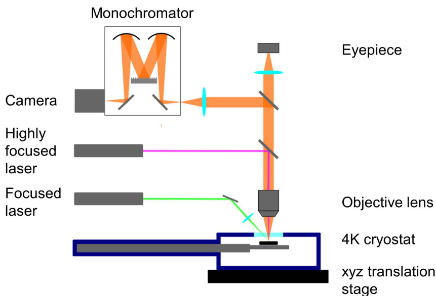
Figure 3.3: Schematic image of a micro PL setup. The laser light can be focused by a lens from the side or through the objective lens. The eyepiece is used to locate the nanowires and the camera detects the luminescence.
