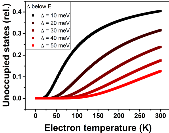
Figure 2.4: Temperature dependence of the fraction of unoccupied states selected energies below the Fermi energy.
