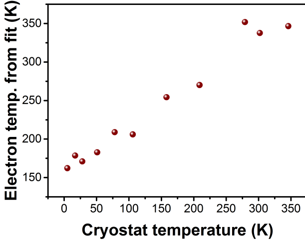
Figure 4.8: Cryostat temperature dependence of the electron gas temperature in n-doped InP nanowires, estimated through a fitting procedure of the PL spectra assuming a Fermi-Dirac distribution of the conduction band electrons in a parabolic isotropic conduction band.
