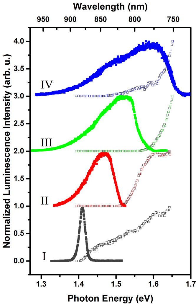
Figure 4.4: Low temperature PL (filled squares) and PLE spectra (hollow squares) of individual nanowires normalized to the same maximum intensity. (I) A nominally undoped nanowire and from (II) to (IV) nanowires with increasing doping concentration. The doping concentration of spectrum IV is comparable to the the doping for the red spectrum in Figure 4.2. The detection energy for the PLE was at 1.38 eV.
