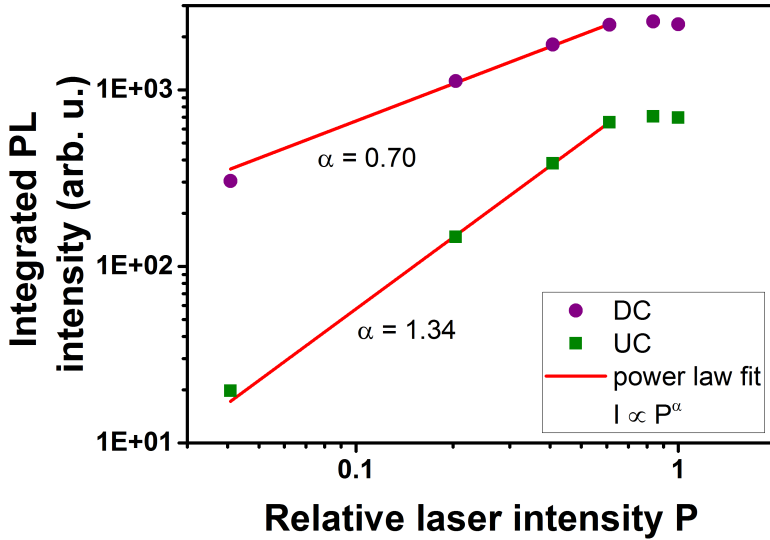
Figure 4.15: Excitation intensity dependence of integrated upconversion (UC) and downconversion (DC) intensity of n-doped InP nanowires for 840 nm (1.48 eV) laser excitation, measured at 4 K.
