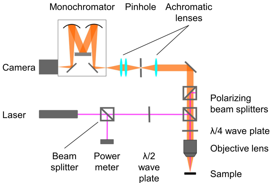
Figure 3.4: Schematic image of the cross-polarized dark field PL setup. The \lambda/2 wave plate is used to adjust the laser light polarization to the alignment of the polarizing beam splitter cubes. The combination of polarizing beam splitters, achromatic lenses and pinhole strongly suppresses the laser light intensity in the monochromator and the camera.
