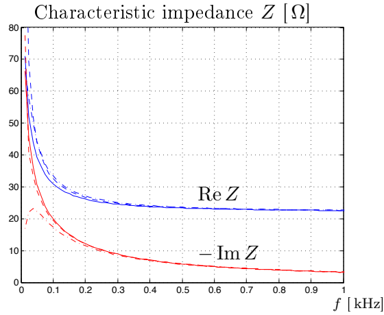
Figure 14: Parameter study with regard to the impedance characteristics of the power cable TM 01 mode over the frequency range 0–1 kHz. The blue lines show \text{Re } Z and the red lines show -\text{Im } Z . The exterior parameters are (\epsilon_{r8}, \sigma_8) = (1, 0) (solid lines), (\epsilon_{r8}, \sigma_8) = (80, 0) (dashed lines) and (\epsilon_{r8}, \sigma_8) = (80, 1) (dash-dotted lines).
