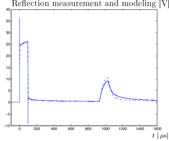
Figure 9: Comparison between measurement data (solid line) and modeled response (dashed line) based on the quasi-TEM mode TM_{01} . A rectangular pulse with duration 100 \mu\text{s} was transmitted at t = 0 and the reflected pulse was received at about 930 \mu\text{s} .
