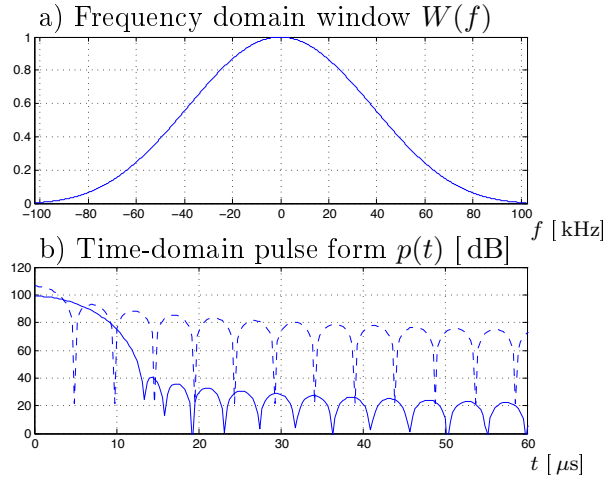
Figure 6: Illustration of frequency domain windowing and time-domain resolution and dynamics. The upper plot a) shows the Kaiser window with parameter \beta = 8 for a modeling bandwidth of 100 \text{ kHz} . The lower plot b) shows a comparison between the convolving pulse form p(t) (plotted here as 20 \log |p(t)| in dB) obtained from the Kaiser window (solid line) and a rectangular window (dashed line).
