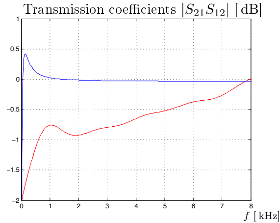
Figure 16: Magnitude of the transmission coefficients |S_{21}S_{12}| . The blue line is based on the single-mode transmission line model and the red line on the calibrated parameters.
