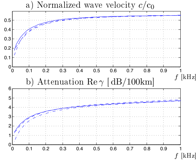
Figure 13: Parameter study with regard to the dispersion characteristics of the power cable TM 01 mode over the frequency range 0–1 kHz: a) Normalized wave velocity c/c_0 = k/\text{Im } \gamma(k) . b) Attenuation 2 \cdot 10^6 \log e \text{Re } \gamma in dB/100km. The exterior parameters are (\epsilon_{r8}, \sigma_8) = (1, 0) (solid lines), (\epsilon_{r8}, \sigma_8) = (80, 0) (dashed lines) and (\epsilon_{r8}, \sigma_8) = (80, 1) (dash-dotted lines).
