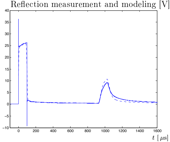
Figure 9: Comparison between measurement data (solid line) and modeled response (dashed line) based on the quasi-TEM mode \text{TM}_{01} . A rectangular pulse with duration 100 \mu\text{s} was transmitted at t = 0 and the reflected pulse was received at about 930 \mu\text{s} .
