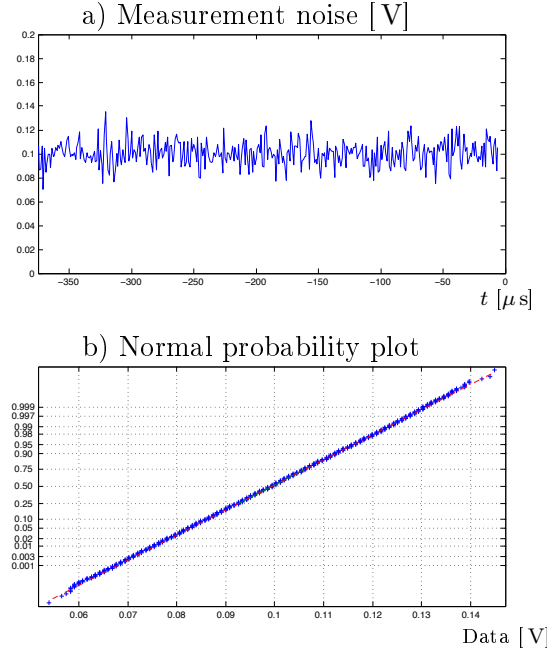
Figure 20: Illustration of measurement noise statistics. The upper plot a) shows 375 \mu s of the measurement noise prior to pulse excitation (decimated here to a sampling rate of 1 MHz). The lower plot b) shows a normal probability plot corresponding to 375 \mu s of the measurement noise at a sampling rate of 500 MHz (187500 data points).
