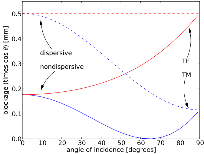
Figure 2: The integrated transmission blockage and its bounds (left and right hand side of (3.9) times \cos \theta ) for a 0.3 mm dielectric sheet. Solid lines are for constant (nondispersive) relative permittivity \epsilon_r = 4.35 , dashed lines are for frequency dependent (dispersive) relative permittivity \epsilon_r(k) = 1 + (4.35 - 1)/(1 - ik/k_c) , using k_c = 2\pi/(1 \mu\text{m}) . The bounds are exactly on top of the simulated transmission blockage. Note the zero transmission blockage for nondispersive case in TM polarization at 64^\circ , corresponding to the Brewster angle.
