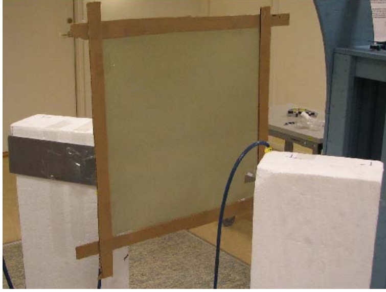
Figure 4: Measurement setup for oblique incidence on an array of split ring resonators. The sheet was oriented with the gaps in the split rings along the vertical direction.
