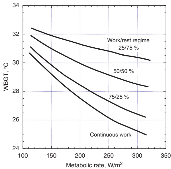
Fig. 1. Recommended work–rest regimes for combinations of metabolic rate ( x -axis) and values for the WBGT-index ( Y -axis). At a work rate of 210 W/m 2 and a WBGT of 30°C a 1-hour shift should be split into 30 minutes of work and 30 minutes of rest. Modified from ISO 7243.
