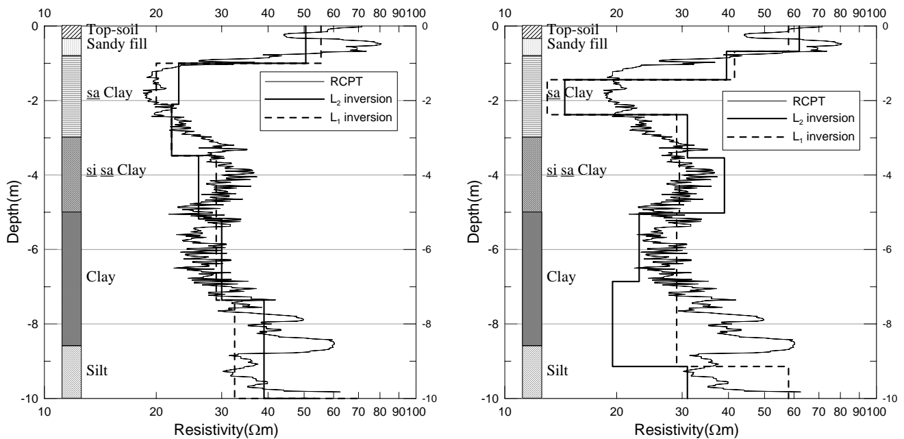
Figure 3. Example data from the Bara test line. Comparison between RCPT, extracted resistivity models from least-squares ( L_2 -norm) and robust inversion ( L_1 -norm) and auger drilling documentation: a) Wenner-Schlumberger, b) dipole-dipole.
