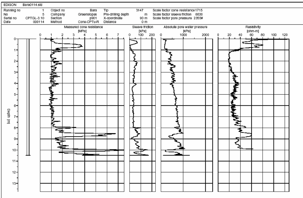
Figure 2. CPT results from distance 90 metres on Bara test line, including measured cone resistance, sleeve friction, generated absolute pore water pressure (atmospheric pressure = 100 kPa) and resistivity.
