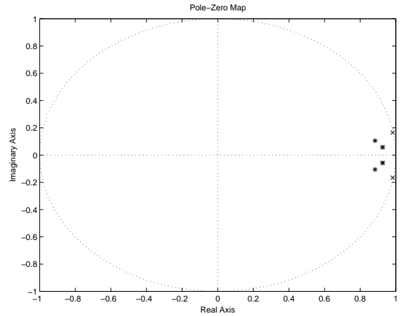
Fig. 11. The open loop poles ( \times ) and the closed loop poles ( * ) (4th order model).
