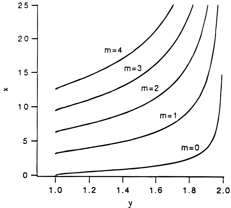
Figure 1: The different x_m(y) curves for \epsilon = 2 .
