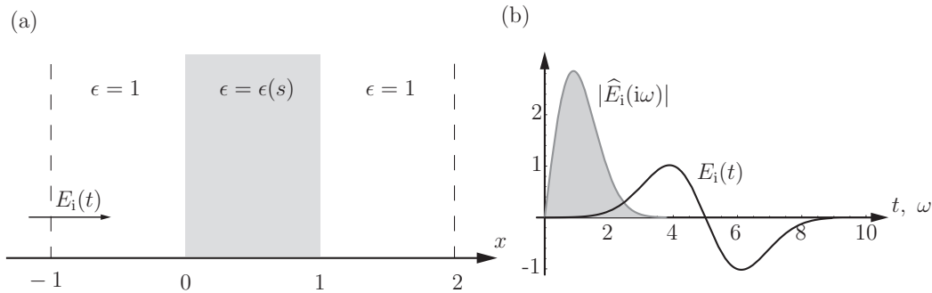
Figure 6: The slab geometry. (a) An electromagnetic field, in vacuum impinges at a dielectric slab from the left. (b) The temporal and spectral behavior of the incident field.
