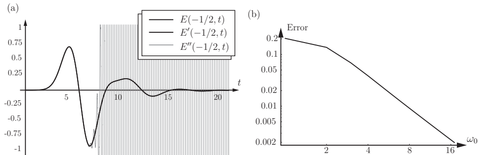
Figure 8: The scattered fields in the slab problem. (a) shows the electric fields at x = -1/2 for the constitutive maps (6.1), (6.2), and (6.3). The fields of the first approximation approximate the original fields well (the error is of the order 0.1% as seen in (b)) whereas the fields of the second approximation give a bad approximation due to the exponential growth rate of the fields. Observe that the field values are cut for values larger than 1 and, hence, the exponential growth rate of the second approximation E'' is not shown in the figure. (b) shows the error of the first approximation as a function of the resonance frequency \omega_0 . Observe that the error decays as \omega_0^{-2} as predicted (4.22).
