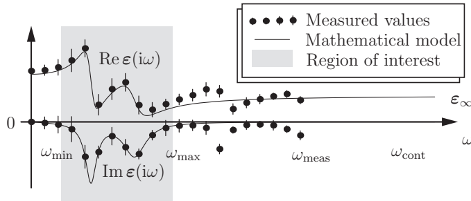
Figure 1: Illustration of the range of validity of the constitutive relations. The measured values of the constitutive map \varepsilon are given up to frequency \omega_{\text{meas}} , the mathematical model is used for frequencies in the interval [\omega_{\text{min}}, \omega_{\text{max}}] , and \omega_{\text{cont}} is the upper limit for the use of a continuum model of the medium, respectively.
