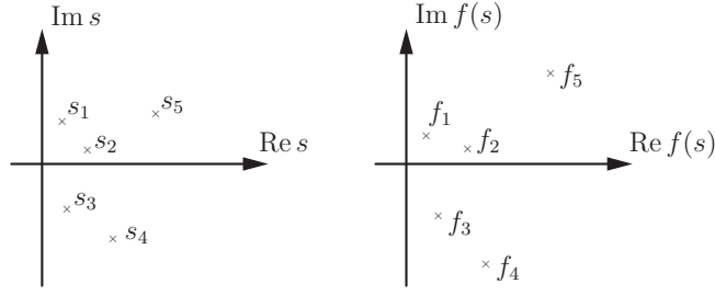
Figure 5: Example of the Nevanlinna-Pick interpolation problem. A function f(s) , analytic in \mathbb{C}_+ , is constructed such that f(s_i) = f_i and \operatorname{Re} f(s) \geq 0 for s \in \mathbb{C}_+ .
