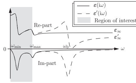
Figure 3: Illustration of the approximation of the constitutive relations. The original constitutive map \boldsymbol{\varepsilon}(i\omega) with the instantaneous response \boldsymbol{\varepsilon}_\infty is approximated by the constitutive map \boldsymbol{\varepsilon}'(i\omega) with the instantaneous response \boldsymbol{\varepsilon}'_\infty < \boldsymbol{\varepsilon}_\infty . The error of the approximation approaches zero in the region of interest [0, \omega_{\max}] as the approximation parameter \omega_0 \rightarrow \infty .
