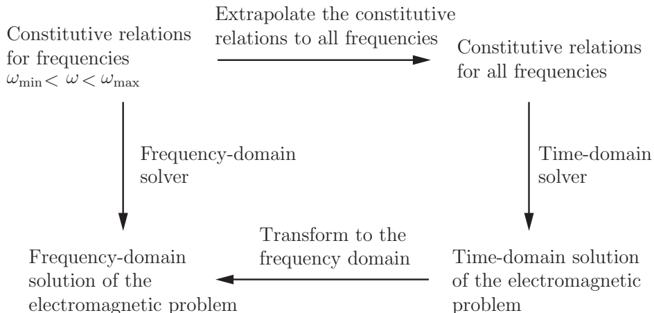
Figure 2: An electromagnetic problem can either be solved in the frequency domain or in the time domain. In the time-domain solution, the definition of the constitutive relations are first extended to all frequencies, or equivalently to the time domain. A time-domain algorithm followed by an inverse Fourier transform gives the desired frequency-domain solution of the original problem. In this paper, we study how the constitutive relations can be extrapolated such that the time-domain approach can be used to give the frequency-domain solution.
