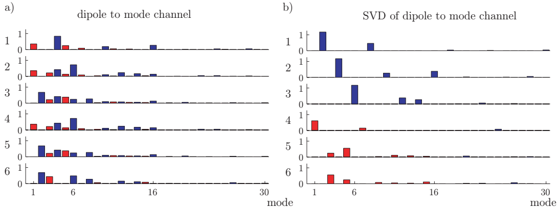
Figure 9: Mode representation of the MIMO tetrahedron with size 0.3\lambda for the first 30 modes, where (5.7) is used to order the modes. a) The mode representation for each dipole, i.e. , each graph represents one column of \mathbf{H}_T and the mode numbers represent the rows of \mathbf{H}_R . b) The mode representation of the orthogonal channels i.e. , the rows and columns of \Sigma \mathbf{V}^H . The first three and last three channels are dominated by electrical dipoles (odd modes) and magnetic dipoles (even modes), respectively.
