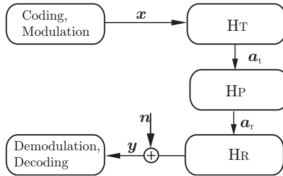
Figure 1: Block scheme of a wireless communication system. The output is \mathbf{y} = \mathbf{H}\mathbf{x} + \mathbf{n} , where the channel is decomposed into the parts \mathbf{H} = \mathbf{H}_R\mathbf{H}_P\mathbf{H}_T and \mathbf{n} is the noise.
