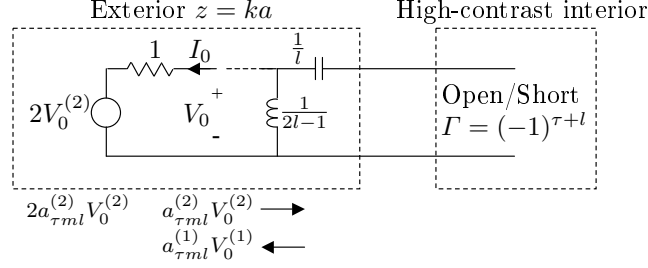
Figure 10: Interpretation of the scattering model in the high-contrast limit, \epsilon(0) = \mu(0) \rightarrow \infty . The exterior circuit is drawn for TM l waves. The TE l waves are similar.
