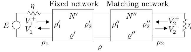
Figure 2: Cascade of two reciprocal two-ports N' and N'' . Here, \rho_1 , \rho_2 and \varrho denote the overall scattering parameters.
