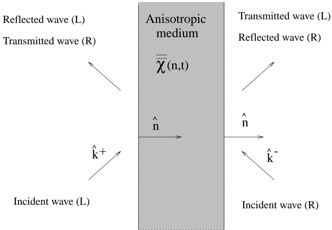
Figure 2: The geometry of the mirror image scattering experiments with incident fields along \hat{\mathbf{k}}^\pm . The scattering experiments are labeled L and R for left and right respectively.
