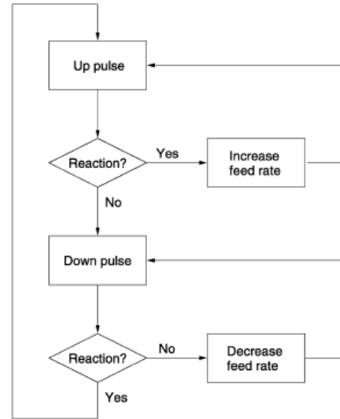
Fig. 3. Illustration of the algorithm used to determine the direction of pulses and changes in F after pulses (Åkesson [1999]).
