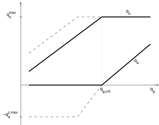
Fig. 1. Oxygen uptake rate q_o , acetate production rate q_a and acetate uptake rate q_a^c plotted against glucose uptake rate q_g . This shows the saturation in the oxidative capacity of the system which occurs when q_g reaches the critical glucose uptake rate for overflow q_{g,crit} . The dashed lines illustrate uptake of acetate.
