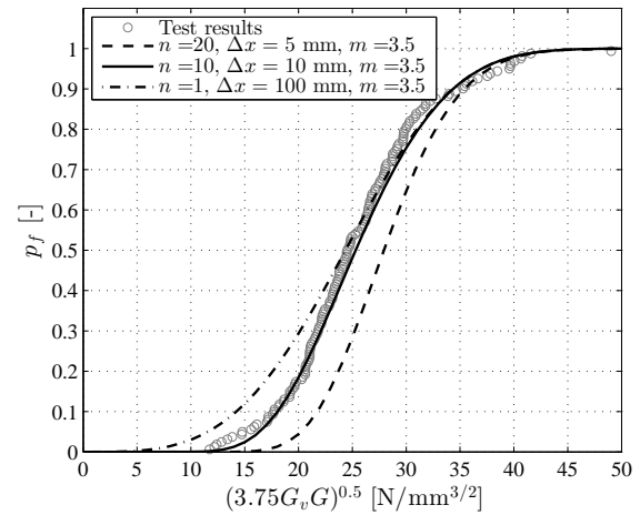
Figure 6: Representation of test results on notched beams (Jockwer, 2014) by the model in Eq. 5 for number of links n of length \Delta x .
