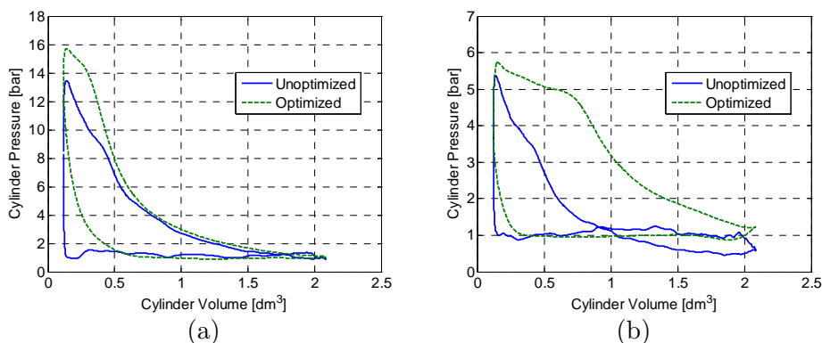
Figure 81 PV-diagram illustrating the cylinder pressure as a function of cylinder volume for the unoptimized and the optimized case during air-motor operation; (a) Tank pressure = 16.5 bar, (b) Tank pressure = 6.5 bar
