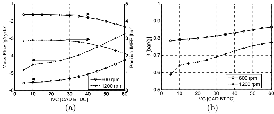
Figure 89 Various parameters as functions of IVC at a tank pressure of 20 bar; (a) Mass flow and IMEP, (b) \beta - the ratio between IMEP and mass flow shown in (a).
