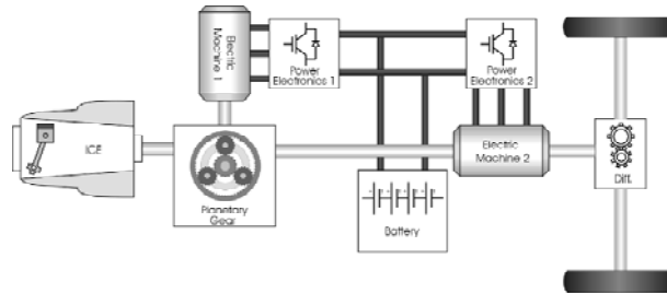
Figure 5 Illustration of a power-split hybrid drivetrain [19]
