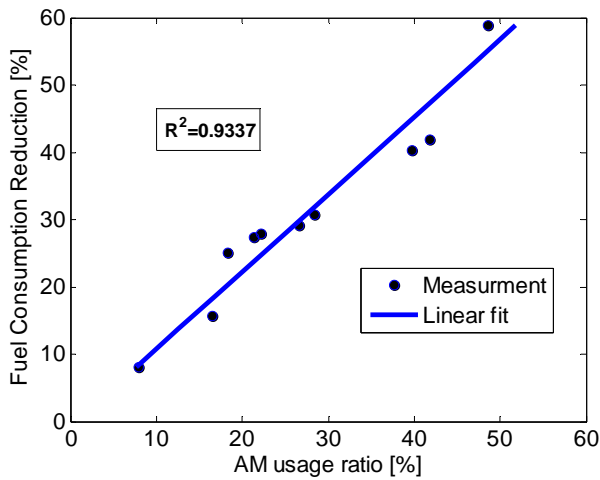
Figure 25 Fuel consumption reduction as a function of AM usage ratio.
