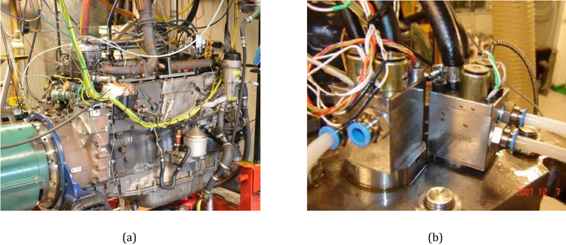
Figure 5 (a) The Engine used in the study. (b) The pneumatic valve actuators mounted on top of the modified Scania cylinder head
