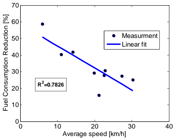
Figure 22 Fuel consumption reduction as a function of average speed
