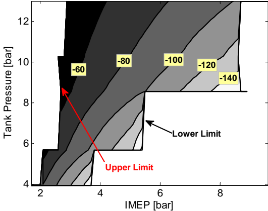
Figure 4 Tank valve opening as a function of both IMEP and Tank pressure. The valve opening is expressed in CAD ATDC.
