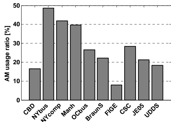
Figure 24 AM usage ratio for different drive cycles
