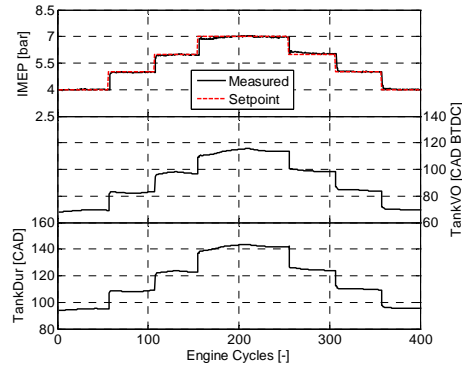
Figure 71 Closed loop process response to several set point changes in IMEP during compressor mode operation at a steady-state tank pressure of 10 bar.
