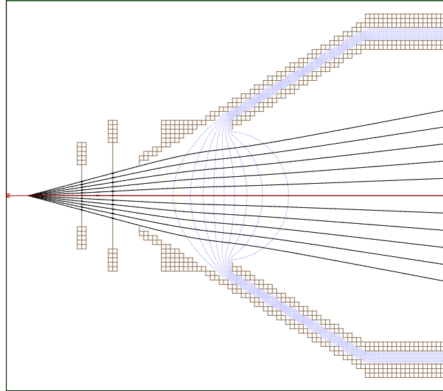
Figure 5.4. Electrostatic simulation of the front gate mounted on the pre-lens. The isolating mounting of the gate is not included as they only have minor effect on potentials. The simulation is cylindrically symmetric. A positive potential equal to the electron kinetic energies is applied to L1. Potential surfaces are shown in blue. An electron fan with \pm 15^\circ is emitted from the source position 25 mm from the lens front. The simulation shows that the electric field in this geometry hardly penetrates the lens front opening.
