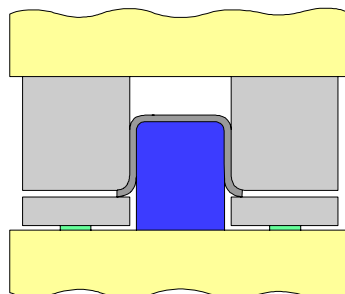
Figure 4.5: Finished part.
