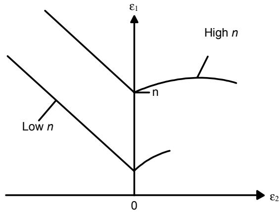
Figure 3.1: Effect of strain hardening on the forming limit curve [58].
