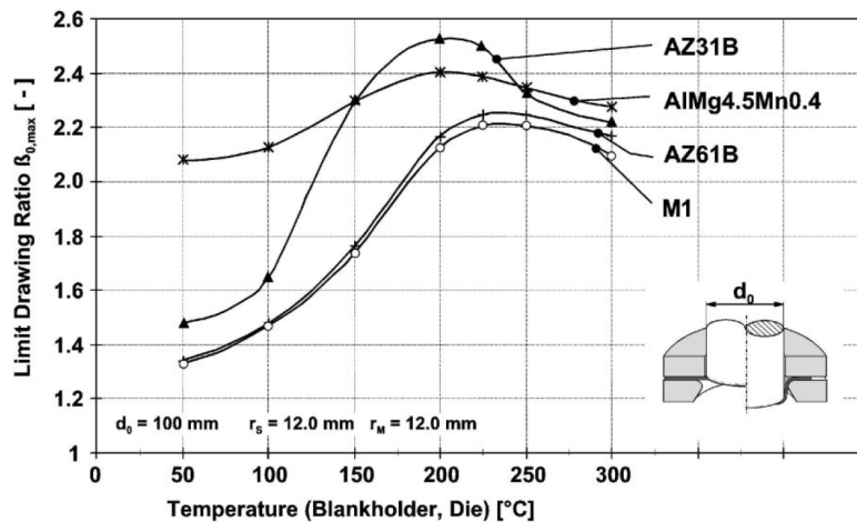
Figure 2.22: Temperature dependent limiting drawing ratios [3].
