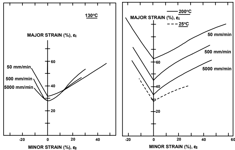
Figure 2.37: Forming limit diagrams for 1.3 mm thick 5182-O, obtained at various temperatures and punch speeds [6].
