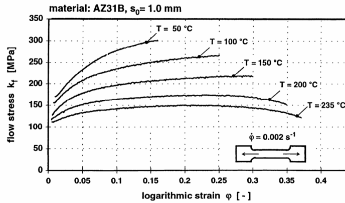
Figure 2.9: Flow curves for AZ31B, sheet thickness 1.0 mm, strain rate 0.002 \text{ s}^{-1} [3].
