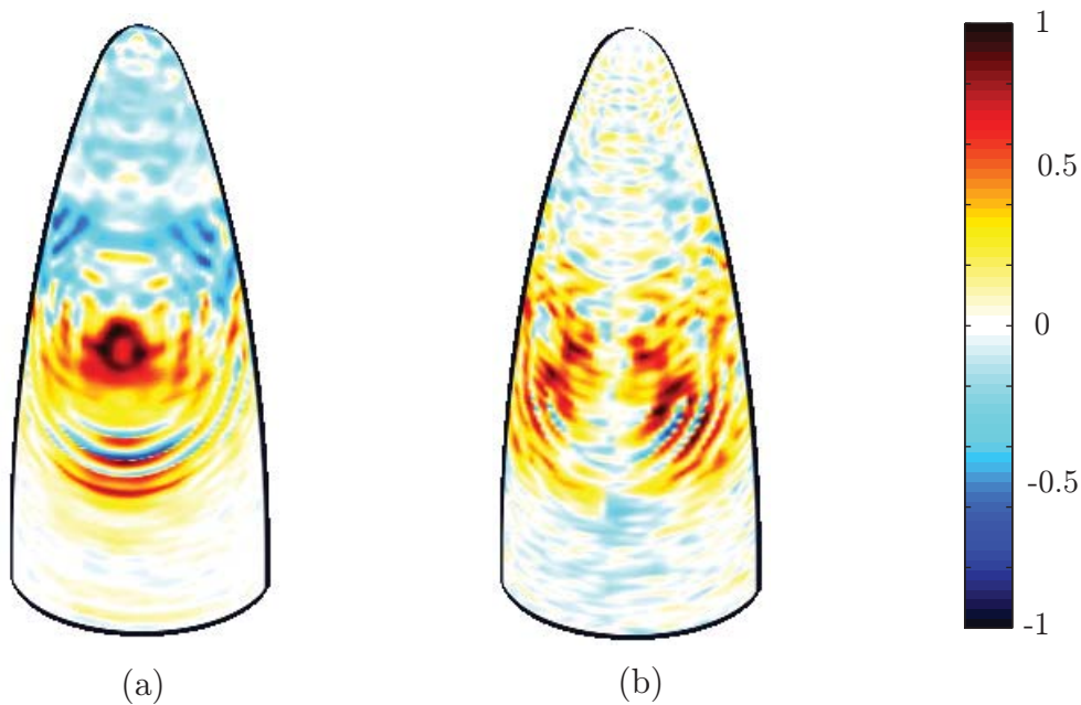
Figure 10: The subtraction between the fields with and without radome present. In (a) (|E_{\text{no radome}}^v| - |E_{\text{radome}}^v|) / \max(|E_{\text{no radome}}^v| - |E_{\text{radome}}^v|) is shown and in (b) (|E_{\text{no radome}}^\varphi| - |E_{\text{radome}}^\varphi|) / \max(|E_{\text{no radome}}^\varphi| - |E_{\text{radome}}^\varphi|) . The front side of the radome, i.e. , the side with the main lobe, is viewed. The scale is linear.
