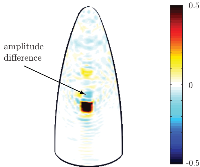
Figure 15: The difference (|E_{\text{radome}}^{\text{v}}| - |E_{\text{def radome}}^{\text{v}}|) / \max\{|E_{\text{radome}}^{\text{v}}| - |E_{\text{def radome}}^{\text{v}}|\} in a linear scale on the front side of the radome. The scale is truncated in order to see the small field amplitude above the copper plate, marked with an arrow.
