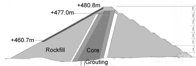
Figure 2. Cross section of the Sädva dam.
