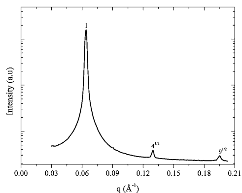
Fig. 5 SAXS patterns from anisotropic samples of the P104/H 2 O/PAA 6000 system. The sample with the composition 49 wt% of P104, 31 wt% of H 2 O and 20 wt% of PAA 6000 (top) was hexagonal showing diffraction peaks at the relative positions 1 : 3 1/2 :4 1/2 :7 1/2 :9 1/2 . The sample with 80.7 wt% P104, 14.3 wt% H 2 O and 5 wt% PAA 6000 (bottom) was lamellar with diffraction peaks at the relative positions 1 : 4 1/2 :9 1/2 .
