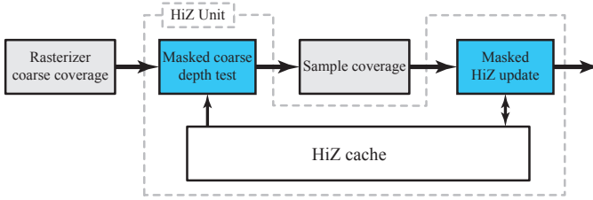
Figure 5: It is possible to modify the coarse depth test to rely only on z_{min}/z_{max} , and not per-sample coverage results. Unlike our solution illustrated in Figure 2 (bottom), this alternative implementation does not incur the expense of per-sample coverage testing prior to HiZ, but can decrease efficiency as culling is performed on more conservative information.
