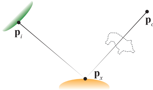
Figure 5: A surface point, \mathbf{p}_x , observed from another point, \mathbf{p}_o . The amount of light reaching \mathbf{p}_o depends the incoming light from all other points in the scene, \mathbf{p}_i , whether there are occluding objects between \mathbf{p}_x and \mathbf{p}_o , on the material of the surface, and on the amount of light that is spontaneously emitted from \mathbf{p}_x .
