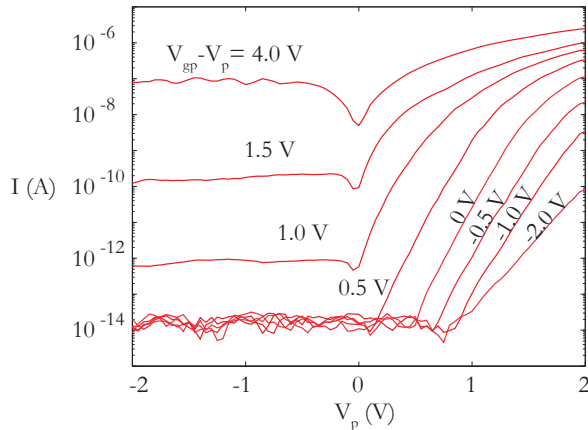
Figure 4.7: The resulting I - V characteristics of the field-effect diode as the p-gate voltage is changed. For V_{gp}-V_p=4\text{ V} both regions are electron-rich and the device allows current to flow in both directions. For V_{gp}-V_p<0\text{ V} the junction acts as a rectifier and the built-in voltage is tuned by the voltage applied to the p-gate.
