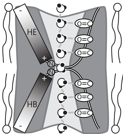
Figure 7. Schematic picture showing the reorientation of water molecules in the pore. On the left side are the half TM helices, showing how their dipole moments result in the positive charge of the electrostatic repulsion filter. Grey lines show how the water molecules hydrogen bond to each other and to the backbone. A reorientation at the NPA boxes breaks this chain of interactions.
