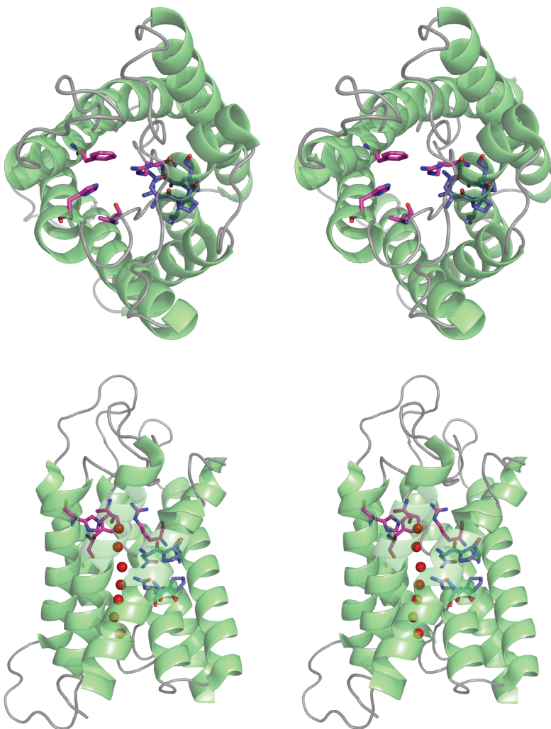
Figure 5. Stereo pictures showing the ar/R filter and NPA motifs. The MIP (HsAQP4, 3GD8) is shown in a green cartoon representation with the ar/R filter and the NPA box motifs shown as sticks in magenta and blue respectively. The upper part shows a top view (from extracellular side) while the lower part shows a side view where parts of helices 4 and 6 are transparent to make the ar/R and NPA regions more visible. The red dots show the positions of waters in the crystal structure.
