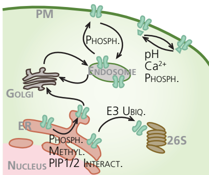
Figure 12. Overview of proposed PIP regulation mechanisms discussed in the chapter.
