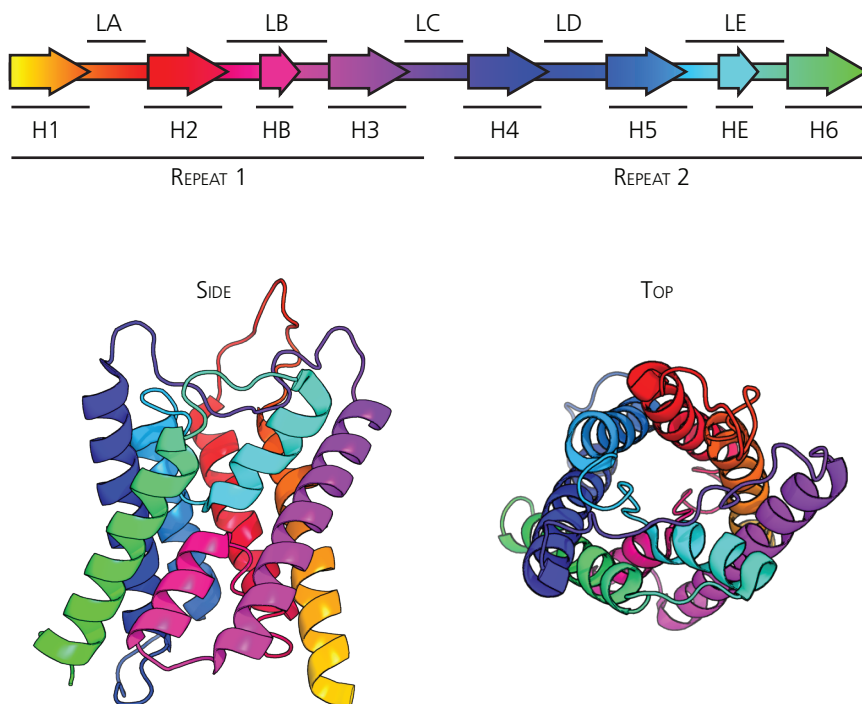
Figure 4. An overview of the MIP Structure. Upper part shows the secondary structure of MIPs, arrows indicate helices. Naming of helices and loops, as well as the positions of the repeats, are indicated. Lower part shows the three-dimensional structure of MIPs from side and top, colored according to the secondary structure cartoon above (The structure is human AQP4, PDBID 3GD8).
