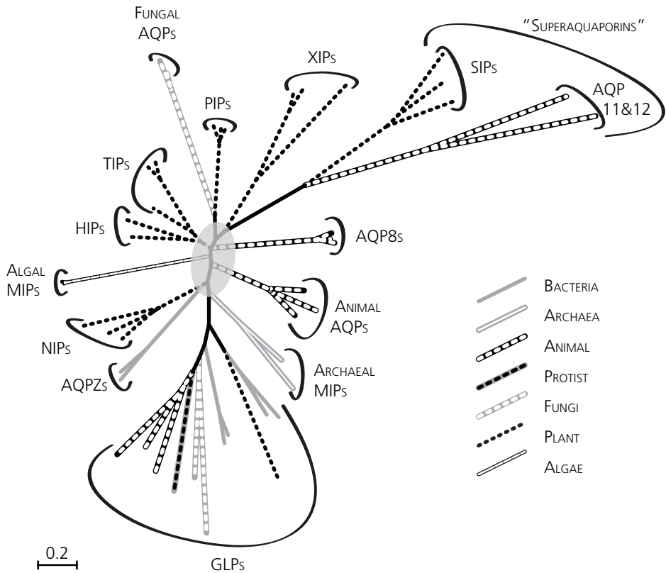
Figure 3. An overview of the phylogeny of the MIP family. A Neighbor Joining (NJ) tree showing the phylogeny of some major MIP subfamilies. Species of MIP sequences are indicated by different line styles and subfamilies are shown by bracketing. The gray shading in the central part of the tree illustrates the uncertainty of the phylogeny of this region indicated by low bootstrap supports in the original analysis.
