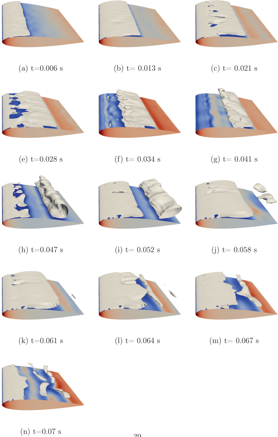
Figure 6.6: Vapour volume fraction \alpha for an uniform nuclei distribution
