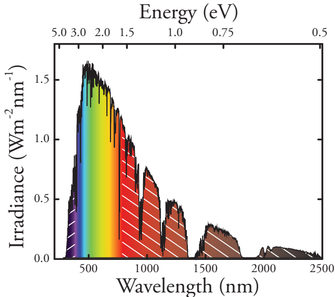
Figure 4.2 AM1.5G reference spectra of sunlight [149] showing the ultraviolet, visible and infrared parts. Light below 300 nm is effectively absorbed in the atmosphere by oxygen, ozone and nitrogen while dips at longer wavelengths are mainly due to absorption by \text{H}_2\text{O} and \text{CO}_2 . The total, un-concentrated, power density is 1000 \text{ W/m}^2 and is often referred to as 1 sun.
