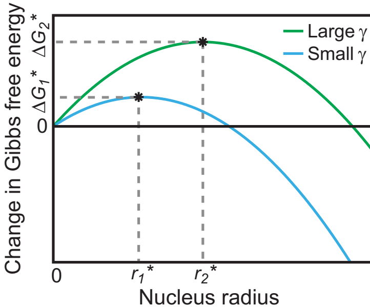
Figure 2.3 Nucleation barrier \Delta G^* for different step energies \gamma . r^* indicates the critical radius after which continued growth is energetically favorable.
