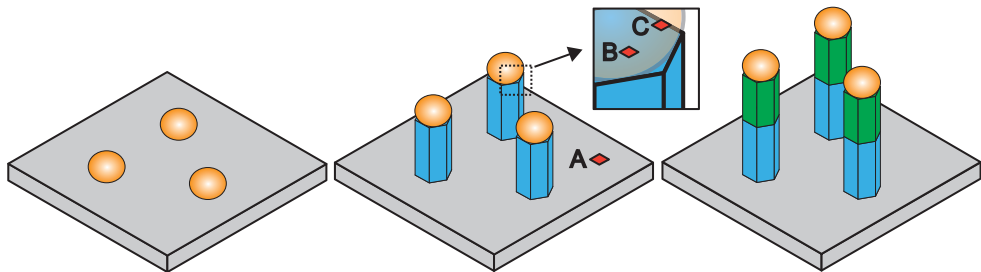
Figure 2.5 Schematic of the particle assisted nanowire growth process. First nanoparticles, typically Au, are placed on a substrate surface. Growth is initiated by the addition of material through the vapour phase. Different sites where nucleation of new crystalline layers can occur are marked as A, B, and C. By switching the precursors, which are supplied through the vapour phase, axial heterostructures or p-n junctions can be formed.
