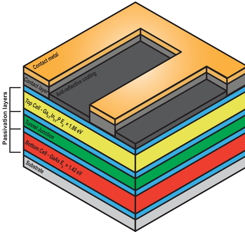
Figure 4.5 Schematic of a tandem solar cell with monolithically integrated sub-cells. Cell structure adapted from ref. [158].
