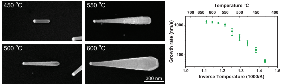
Figure 2.9 SEM images of GaAs nanowires grown by Aerotaxy at different temperatures (left) and the dependence between inverse growth temperature and growth rate (right). The temperature dependence of the growth rate indicates a kinetically limited regime below 550 °C.
