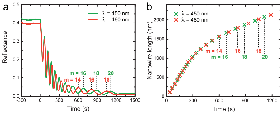
Figure 3.7 (a) Reflectance vs. time for \lambda = 450 nm and \lambda = 480 nm. Growth starts at t = 0 s. (b) Minima and maxima from (a) converted into nanowire length as a function of the growth time by using Eq. (3.2) and the n_{eff} displayed in Figure 3.6b. Some even m numbers have been marked and the data points in (b) can be directly correlated to the maxima in (a).
