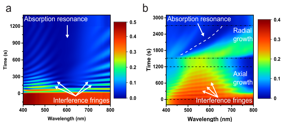
Figure 3.5 Colorplot reflectance spectra obtained from a Laytec EpiR DA UV optical reflectance tool connected to an Aixtron 200/4 MOVPE reactor during growth. (a) Reflectance spectra from axial growth of 130 nm diameter particle assisted InP nanowires with 400 nm pitch as defined by NIL. (b) Reflectance spectra from core and shell growth of selective area InP nanowires with a pitch of 1 \mu\text{m} as defined by NIL. During growth, axial elongation of the nanowires results in the appearance of interference fringes while radial growth causes a shift of absorption resonances.
