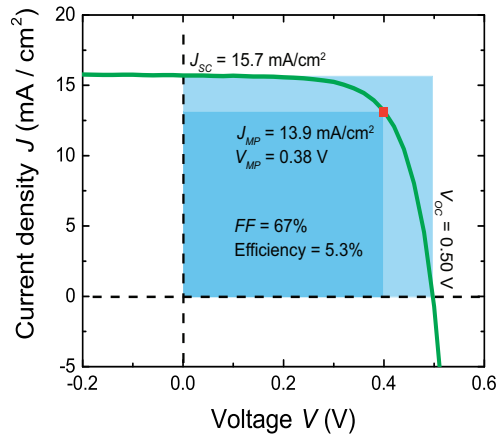
Figure 4.4 J - V curve of a nanowire array solar cell from Paper VIII where the p - n junction was defined in the radial direction. Key performance figures are marked such as the efficiency, FF , maximum power point, J_{sc} and V_{oc} . The incident light consisted of the AM1.5G spectra and had a power density of 1000 \text{ W/m}^2 , equivalent to 1 sun.
