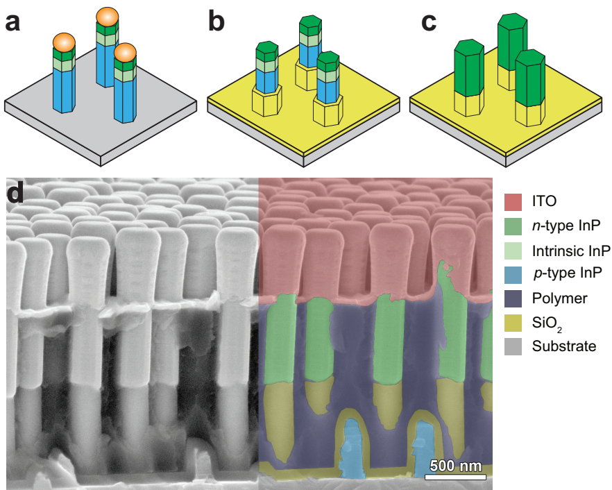
Figure 4.7 (a)-(c) Schematic of the growth process used in Paper VIII. (a) Particle assisted core nanowire growth of a p - i - n structure. (b) The Au particle is removed in a wet etch process and \text{SiO}_2 is deposited by ALD which is subsequently etched back. (c) Regrowth of an i - n shell where the \text{SiO}_2 now masks part of the core. (d) Partially false colored cross section SEM image of a contacted device.
