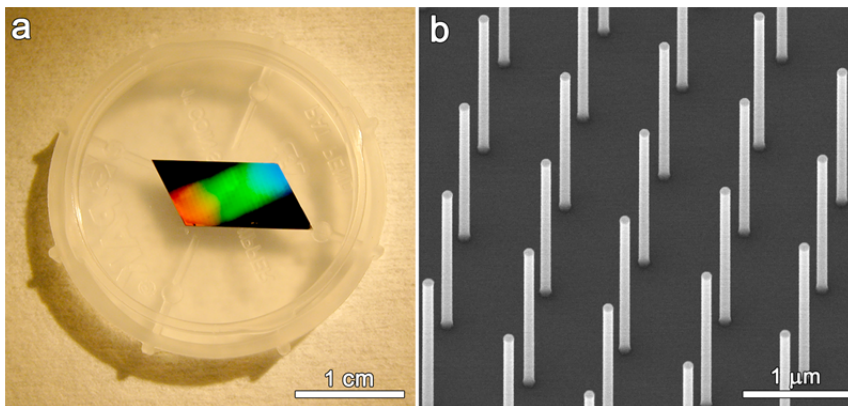
Figure 1.2 (a) Photograph of a sample with nanowires. The nanowires diffract the incoming light resulting in different colors which are visible. (b) Scanning electron microscope (SEM) image of the nanowires in (a) acquired at a tilt angle of 30^\circ . The nanowires are standing vertically from the substrate and are roughly 100 nm in diameter. They are arranged in a periodic pattern with a nanowire-to-nanowire distance, or pitch, of 1 \mu\text{m} .
