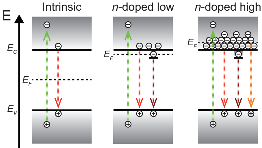
Figure 3.9 Schematic of the recombination processes during a PL experiment in an intrinsic, low n -doped and high n -doped semiconductor. Green light is used to excite electrons from the valence band ( E_V ) to the conduction band ( E_C ) in the semiconductor. Depending on which states the electrons occupy recombination can occur from the conduction band edge, dopant level or within the conduction band. The spectral shape and peak energy of the luminescence changes depending on which recombination processes that occur and can be used to quantify the amount of carriers.
