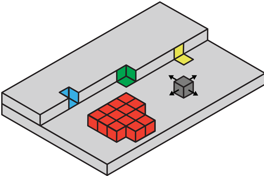
Figure 2.2 Crystal growth illustrated through building blocks. The adatom (dark grey) diffuses on the surface and can incorporate at the step (yellow), kink (green) or step vacancy (blue). The number of faces where the adatom can bind determines how strongly the adatom is bonded. If the diffusion length is smaller than the spacing between the steps, growth can proceed via a “birth and spread” mechanism where a nucleus (red) forms on the flat surface.
