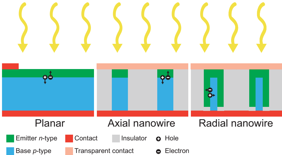
Figure 4.1 Principal structure of a conventional planar, axial nanowire and radial nanowire solar cell. An axial nanowire solar cell is analogous to a planar since charge separation and light propagation occurs in the same direction. In a radial nanowire solar cell charge separation instead occurs orthogonal to the direction of light propagation.
