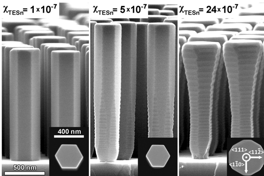
Figure 3.10 Side and top view of three core-shell InP nanowire samples where the shell has been grown with different molarfractions of TESn ( \chi_{TESn} ). A low value of \chi_{TESn} promotes \{1\bar{1}0\} side facets while higher flows promote formation of \{111\} facets. At a medium flow both types of facets can be observed.
