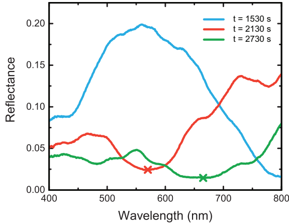
Figure 3.8 Wavelength dependent reflectance spectra during different stages of shell growth extracted from the data in Figure 3.5b, where minimum values used for identifying the nanowire diameter have been marked. The nanowire sample consisted of selective area grown nanowires with a pitch of 1 \mu\text{m} and core diameter of 153 nm. At t = 1530 s (blue line) shell growth starts and the absorption resonance from the HE_{11} mode is only partly visible at 800 nm. At t = 2130 s (red line) the nanowire diameter has increased and the reflectance minima at 572 nm corresponds to a nanowire diameter of 232 nm (absorption from HE_{12} mode). At t = 2730 s (green line) the growth stops and the reflectance minima is found at 659 nm corresponding to a nanowire diameter of 289 nm (absorption from HE_{12} mode) which matches well with the SEM measured value of 285 \pm 11 nm.
