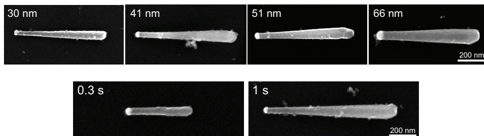
Figure 2.8 SEM images of Aerotaxy grown GaAs nanowires where the Au particle diameter (top) and growth time (bottom) has been changed.
