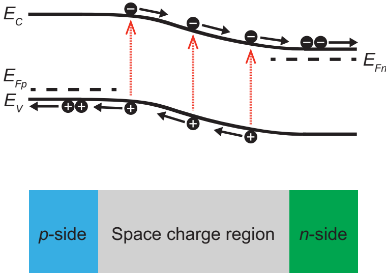
Figure 4.3 Schematic of a p - n junction working as a solar cell. Absorption of light creates electron-hole pairs which are separated in the space charge region giving rise to a drift current.
