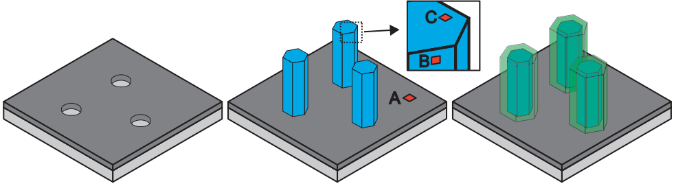
Figure 2.6 Schematic of the selective area nanowire growth process. First an inert mask material, through which holes are etched, is deposited on the substrate surface. Growth is initiated by the addition of growth material through the vapour phase. Different sites where nucleation can occur are marked as A, B and C. By switching the precursors which are supplied through the vapour phase, and other growth parameters such as temperature, heterostructures and p - n junctions in a core-shell geometry can be formed.
