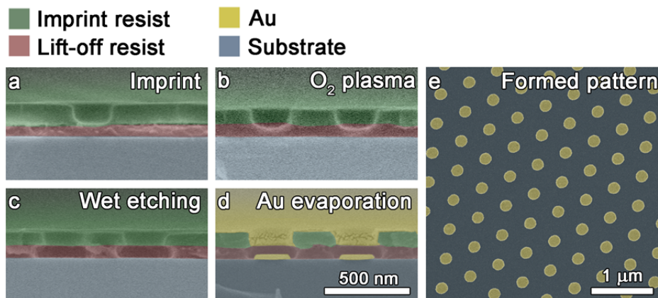
Figure 3.2 Overview of the in-house developed imprint process. (a) An IPS is used to form depressions in the imprint resist but leaves a small residual layer at the bottom of each hole. (b) An O 2 plasma is used to remove the residual layer before (c) a wet etching step creates an undercut profile. (d) Finally Au is evaporated and (e) a remover chemical is used to remove the remaining polymer and unwanted Au, leaving a regular pattern of Au particles.
