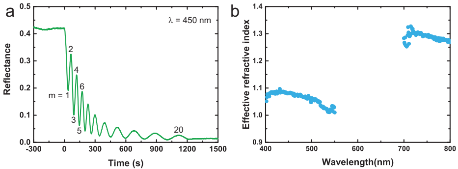
Figure 3.6 (a) Reflectance signal at \lambda = 450 nm from a nanowire growth run where some minima and maxima have been marked with their respective m number. Growth starts at t = 0 s. (b) Effective refractive index n_{eff} of a nanowire array with 400 nm pitch and 130 nm nanowire diameter. Between 550 nm and 700 nm an absorption resonance exists which makes extraction of n_{eff} difficult.
