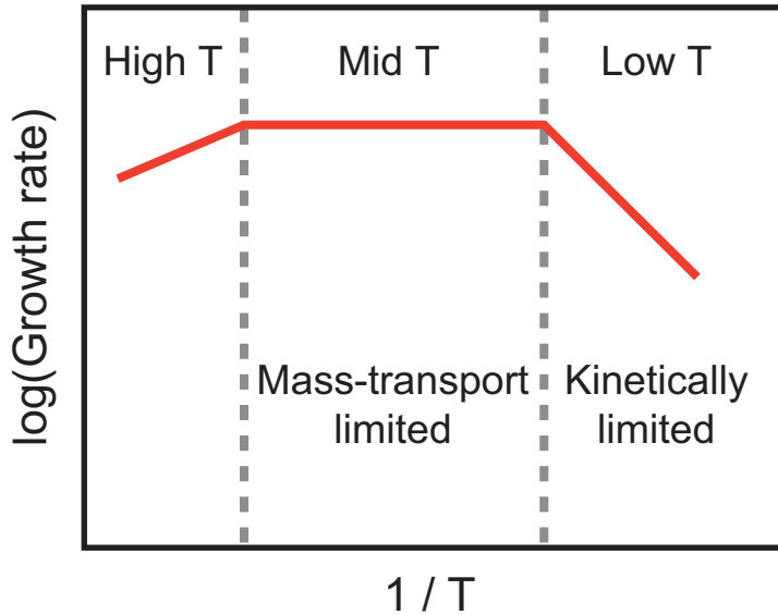
Figure 2.4 Logarithm of growth rate vs. inverse temperature for a typical MOVPE process. For low temperatures reaction kinetics limits the growth and an exponential increase in the growth rate with inverse temperature is observed. At medium temperatures the precursors decompose more readily and the growth rate is temperature independent. The growth rate is instead limited by supply of growth material. At very high temperatures the growth rate is reduced due to for example desorption of growth material from the crystal surface or parasitic reactions in the reactor.
