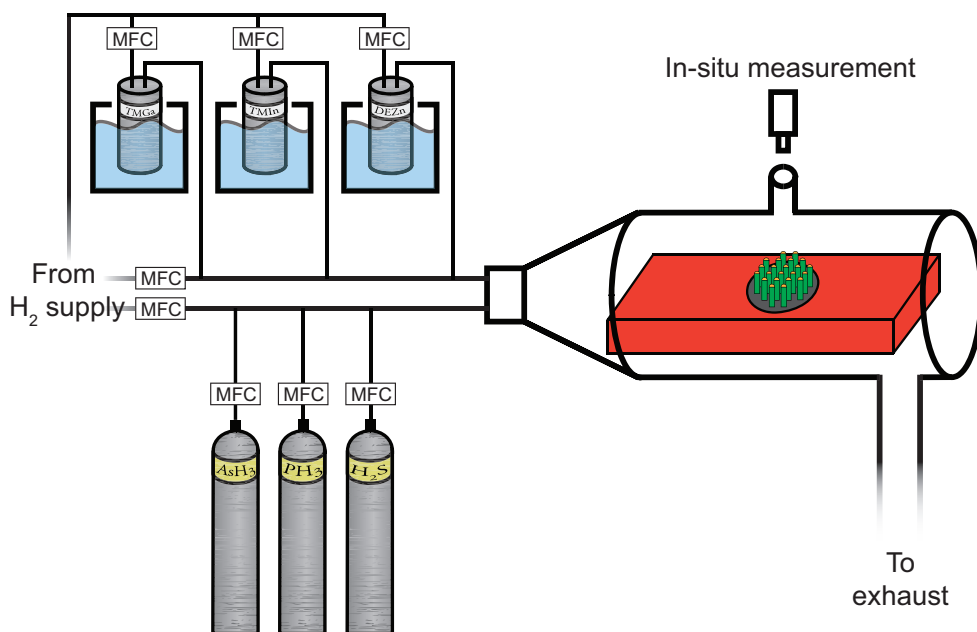
Figure 2.1 MOVPE system with three different metal-organic precursor sources placed in temperature controlled liquid baths and three high vapour pressure hydride sources supplied directly through gas bottles. The gas flows are controlled by mass flow controllers (MFCs). Inside the reactor the substrate (red) is heated which together with the precursor molecules facilitates (nanowire) growth on the substrate. Above the reactor an in situ measurement tool is located which can acquire the optical reflectance spectra of the sample during growth.
