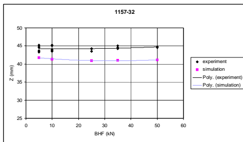
Figure 5. Springback as function of the blank holder force. The diagrams show the results for the extra high strength-steel (Docol 600).
