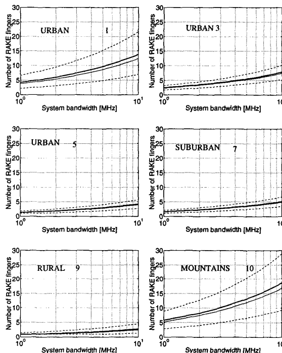
Figure 2. Number of CDMA RAKE fingers needed to track the 90% of the total available power as a function of the system bandwidth. Results are shown for different areas according to Table 1 and equation (3.3). The dashed line corresponds to the 10% and 90% probability level according to eq. (3.3). The thin continuous line corresponds to the 50% and the thicker line is the average (3.4)
