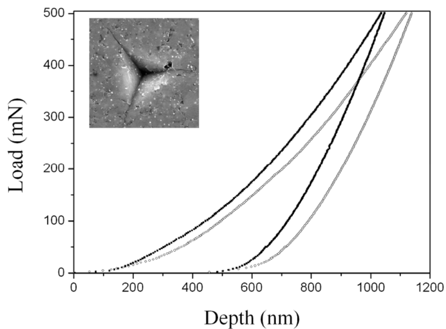
Fig. 3 Characteristic load-displacement curves for bulk boron phosphides BP (open symbols) and B 12 P 2 (solid symbols). Inset: SEM image of the residual imprint formed by Berkovich indenter on the surface of B 12 P 2 sample at 300 mN peak indentation load.
