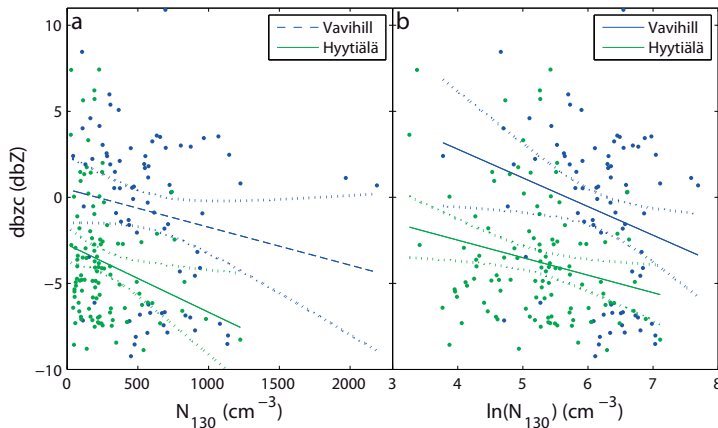
Figure 12 dbzc as a function of N_{130} for precipitating cases only. In b), the natural logarithm was applied to the N_{130} . The dotted lines represent the 95% prediction intervals for the relationships. The solid lines have a statistically significant correlation, the dashed lines have a non-significant correlation and the dotted lines are the 95 % confidence intervals of the relationships (Sporre et al., 2014).
