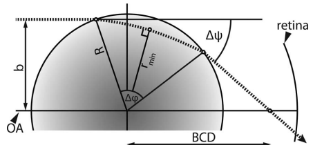
Fig. 1. Trajectory of a ray (dotted line) passing through the lens. R denotes the radius of the lens, while r_{\min} is the distance from the lens center to the point where the ray comes closest to the center. This point is called the symmetry point because the ray's trajectory outward from this point is symmetrically identical to its way inward. \Delta\psi is the total deflection angle, \Delta\phi is the angular extent of the ray's trajectory in the lens, b is the ray's entrance position, which is the lateral distance between the incoming ray and the optical axis, OA, and BCD is the back center distance, i.e., the distance from the lens center to where the beam intercepts the OA.
