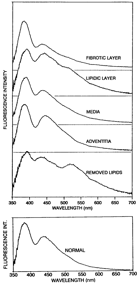
FIGURE 1 A: Fluorescence spectra from different layers of an atherosclerotically diseased vessel wall using nitrogen laser excitation (337 nm). The samples are from top to bottom: fibrotic layer, lipid-rich yellow layer, non-diseased media, adventitia and lipid-rich yellow substance removed from the plaque. B: Fluorescence spectrum from the surface of a non-diseased piece of an aortic vessel wall. The excitation wavelength was 337 nm.
