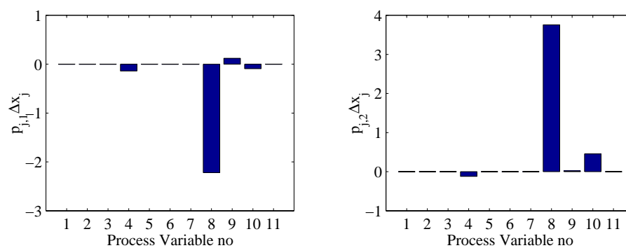
Figure 8.4 Variables contributing to change along PC no 1 (left) and PC no 2 (right).
