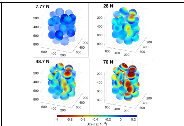
Fig. 2: Strain tensor data for each of the grains, in a sample of quartz grains (sample width is about 1.5 mm), presented as a 3D rendering of the strain ellipsoids onto the 3D grain surfaces from x-ray tomography (in the initial configuration) at different axial loads; see [7] for more details.
