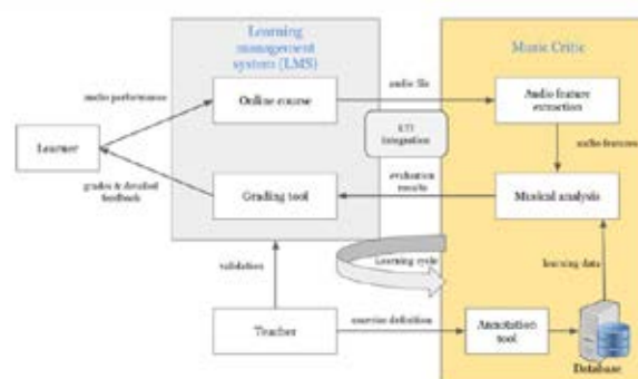
Figure 1: Music education workflow based on the MusicCritic framework
