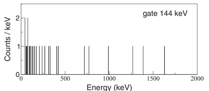
FIG. 3. Gamma-ray spectrum in prompt coincidence with the 144-keV transition from the decay from the isomeric state in ^{211}\text{Tl} .
