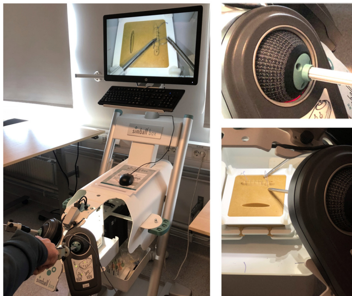
Figure 4. Simball® Box simulator. Upper right, laser-marked pattern which allow instrument tracking. Lower right, suture pad exercise. Photo by KH 2018
