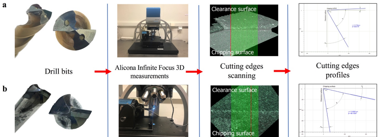
Fig. 2. Drill bits cutting edges scanning; (a) cemented carbide drill bit; (b) PCD drill bit.
