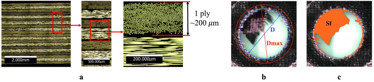
Fig. 1. (a) Structure of Saab CFRP; (b) delamination evaluation; (c) uncut fibers evaluation.
