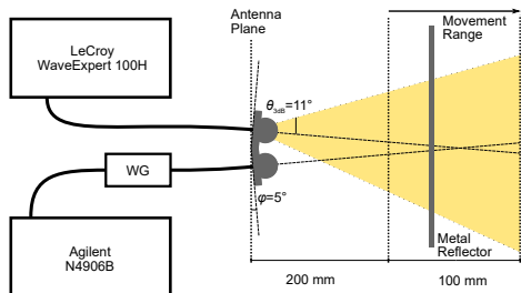
Fig. 1. The used reflectometry setup. A 300x300 mm big metal mounted on a translational stage in a distance of 200 mm from a pair of wideband leaky lens antennas ( \theta_{3dB} = 11^\circ at 60 GHz). The reflector is swept over a distance of 100 mm and the reflection is recorded.
