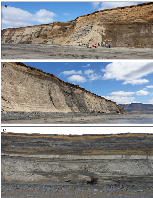
Figure 2. The Melabakkar-Ásbakkar coastal cliffs. A: Thrust stacked and folded glaciomarine diamicton, sand and gravel within the Ás moraine. Displacement was from the north (from left to right). The deformed sediments are overlain by laminated, glaciomarine silt and sand. B: Undeformed, bedded/laminated glaciomarine sediments exposed in Melabakkar-Ásbakkar. The height of the section is around 25 m. C: Thrust stacked and faulted glaciomarine sediments within the Melaleiti moraine. The deformed sediments are unconformably overlain by a sequence of undeformed glaciomarine and littoral deposits
