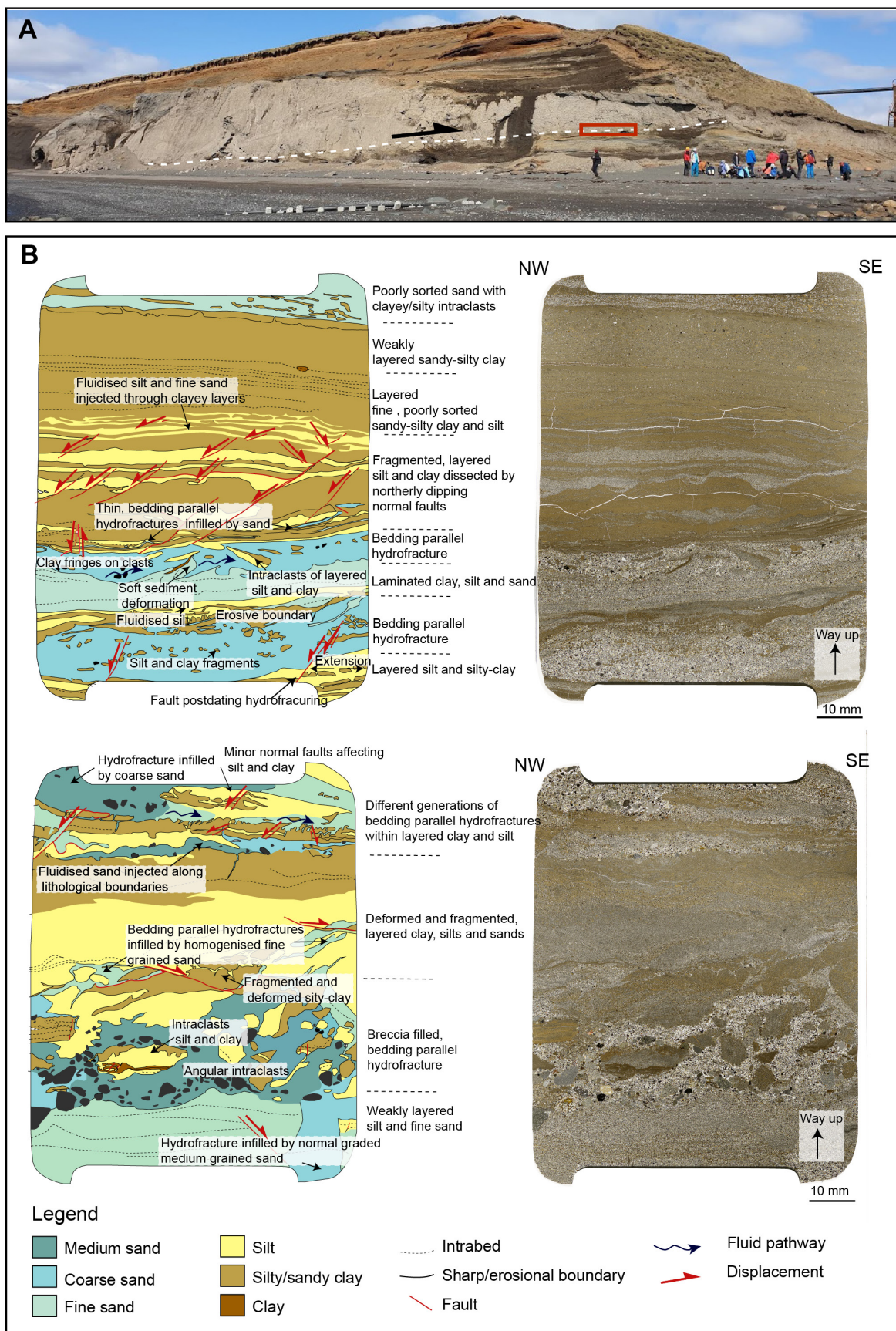
Figure 9. A: The Ásgil thrust block moraine, exposed in the central part of the Melabakkar-Ásbakkar coastal cliffs. The moraine is composed of stacked blocks of glaciomarine silts and sands that have been emplaced upon stratified sand and gravel. It is unconformably overlain by undeformed, post-glacial sediments. The red box shows the sampling site of the thin sections in B and the dashed lines indicate the basal detachment. B: Interpretation diagrams and scans of two thin sections collected close to the leading edge of the moraine. The thin sections show that the base of the thrust block is dissected by erosive sand layers representing sediment liquefaction and hydrofracturing. Only minor shearing is detected indicating that the thrust block was decoupled during its transport supported by overpressurised water along its base.
