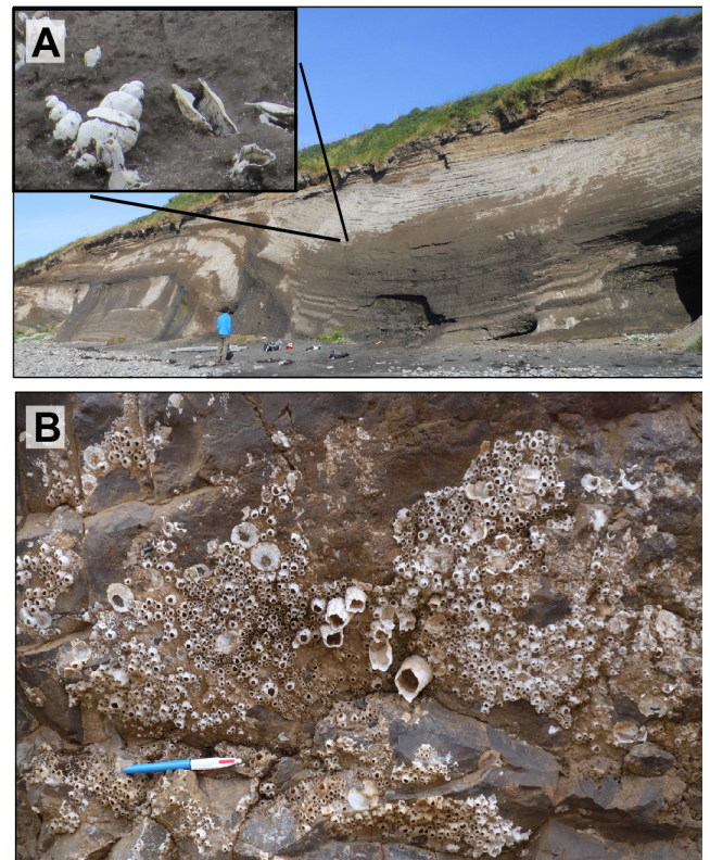
Figure 7. A: Folded and laminated glaciomarine silts and sands in the Belgsholt coastal section (Fig. 1B). These sediments contain well-preserved molluscs that were sampled for radiocarbon dating. B: Balanus balanus shells attached to raised sea cliff at around 70 m altitude at Fossamelar in the mouth of Skorradalur (see locations in Fig. 1B).
