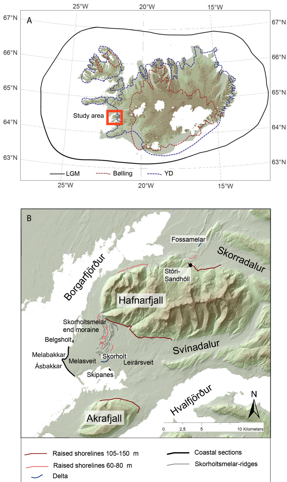
Figure 1. A: The evolution of the Icelandic Ice Sheet (IIS) during the Late Weichselian. The Last Glacial Maximum (LGM: c. 25-20 cal. ka BP) limit is drawn according to Patton et al. (2017) and is based mainly on submarine geomorphology. The suggested minimum ice extent at the end of the Bølling interstadial (c. 14.0 cal. ka BP) and the Younger Dryas maximum extent (YD: c. 12.7-11.5 cal. ka BP) is based on Norðdahl et al. (2008). It is, however, worth noting that the extent of IIS in many parts of Iceland, including western Iceland, is both temporally and spatially poorly constrained. B: A topographic map of the lower Borgarfjörður region, showing localities and the main geological features referred to in the text. The 60-80 m raised shorelines are drawn according to a reconstruction in Ingólfsson (1988), the 105-150 shorelines are drawn according to Magnúsdóttir and Norðdahl (2000) and Ingólfsson & Norðdahl (2001). The map excludes younger shorelines at lower levels. Basemaps from the National Land Survey of Iceland (Landmælingar Íslands).
