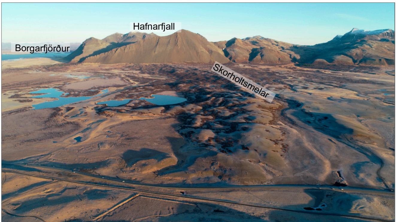
Figure 3. The Skorholtsmelar end moraine. Photo: Ágúst Guðmundsson.
