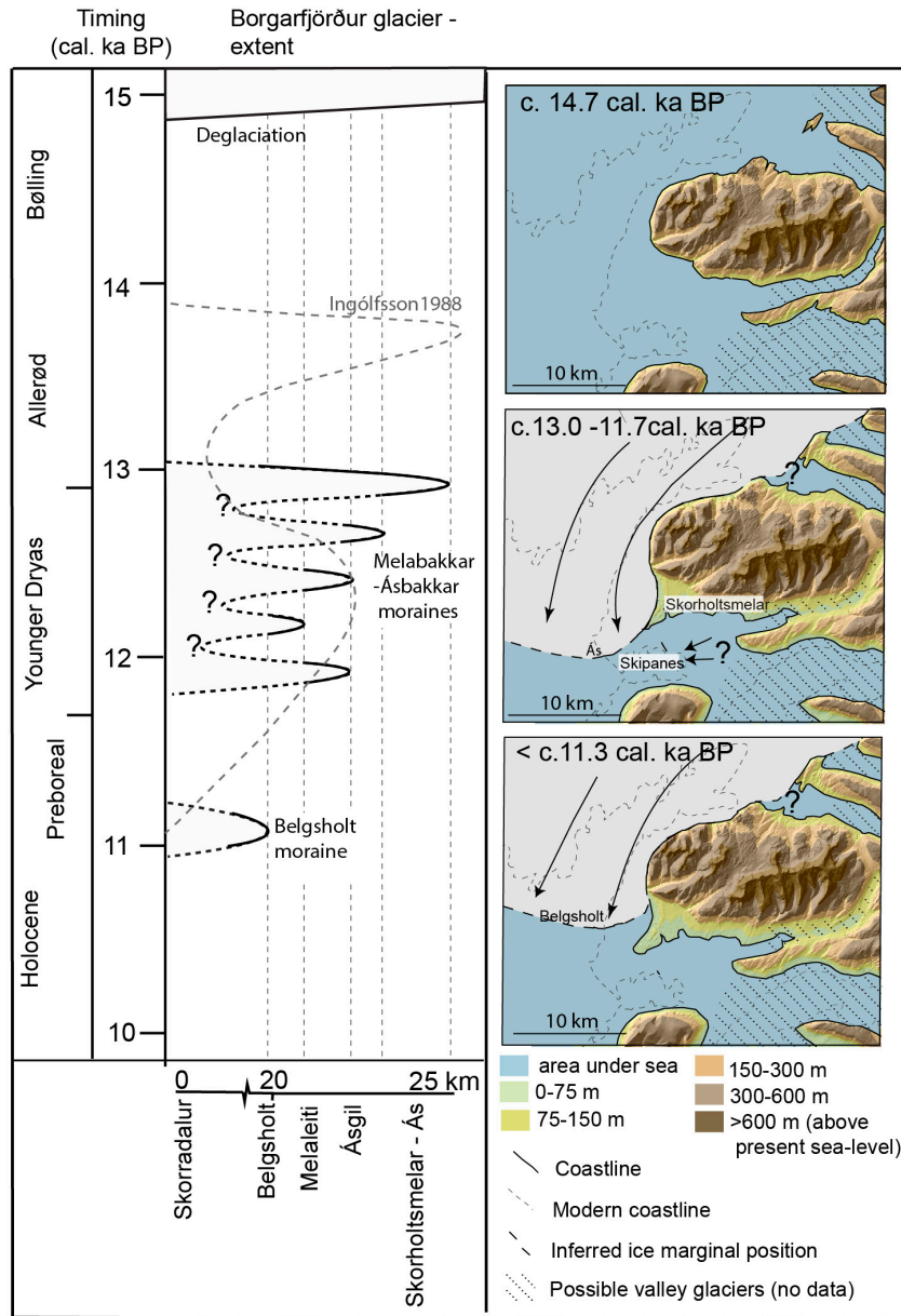
Figure 10. A time-distance model of the advances and retreats of the Borgarfjörður glacier during the Late Weichselian and Early Holocene. The question marks represent unknown ice-marginal position. The schematic time slices show the reconstructed aerial extent of the Borgarfjörður glacier and the approximate sea level position during three different time intervals. The reconstructions are based on radiocarbon ages, altitude of raised shorelines, geomorphology, stratigraphic and glaciotectonic studies. Mountain glaciers are likely to have been present during this time but as their size is unknown they are not drawn. Figure modified from Paper III.
