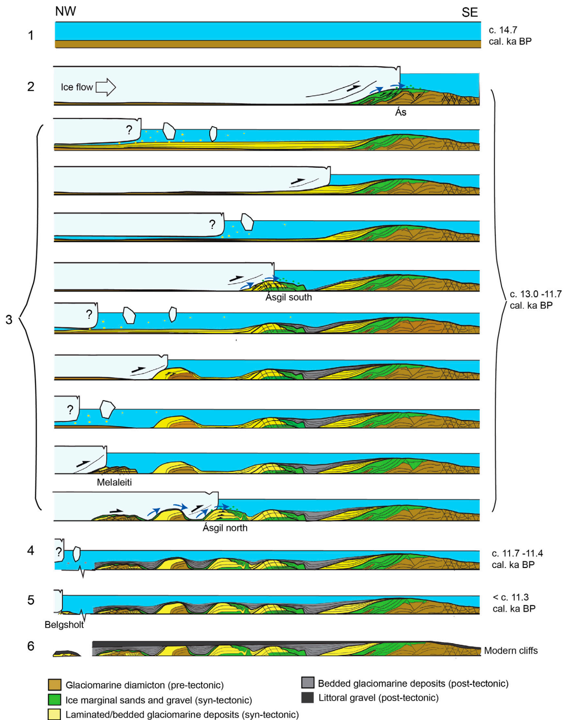
Figure 11. A sequential model demonstrating the formation of the glaciotectionic moraines exposed in the Melabakkar-Ásbakkar. The sequence of events is described in section 7.1. Black arrows indicate displacement and blue arrows indicate water flow. Figure modified from Paper I.
