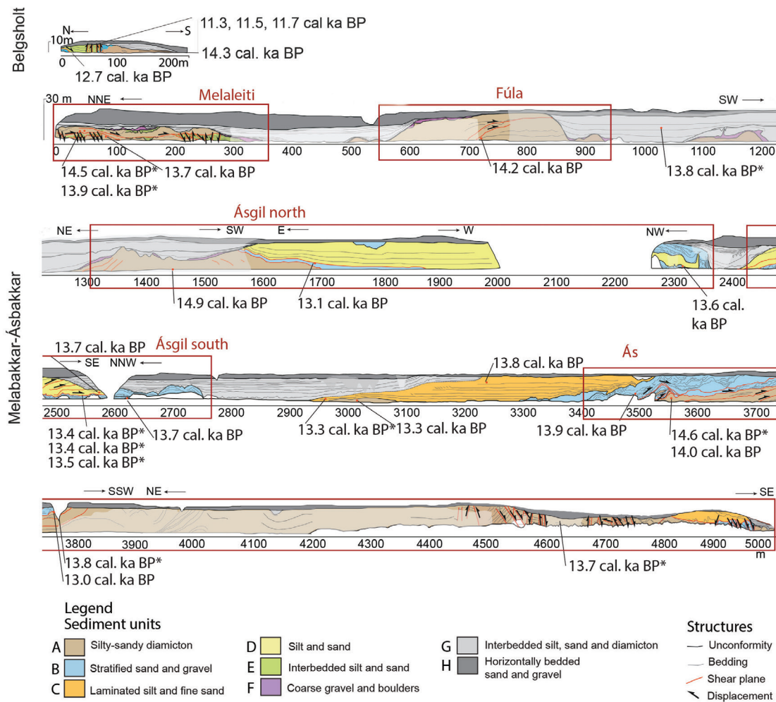
Figure 8. A scale diagram of the Melabakkar-Ásbakkar coastal cliffs based on LiDAR scans and photographs. The drawing is vertically exaggerated (2x). The shaded areas indicate parts of the section that were wet or covered in thin debris that hampered detailed analysis. Units A-E are deformed and form the moraines while Units F-H are undeformed and overly the moraines. The locations of the glaciotectonic moraines in the cliffs are outlined with red boxes. Calibrated radiocarbon ages of shells sampled from the cliffs are marked in the diagram indicating maximum ages of the sediments and the deformation. Ages marked with an asterisk are from Ingólfsson (1987). Figure modified from Papers I and III.
