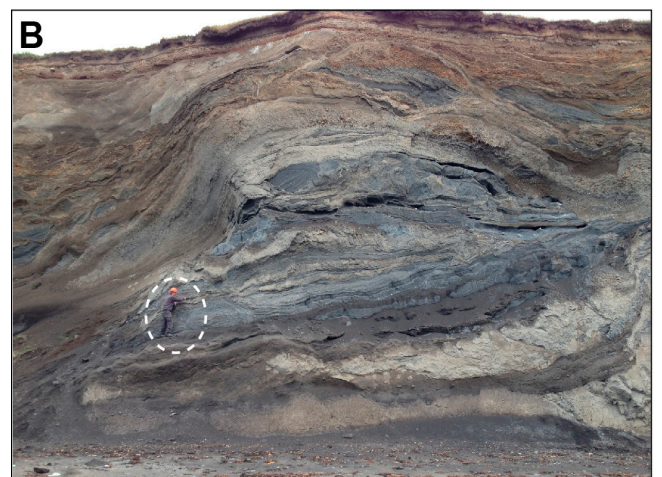
Figure 4. A: Measurement of strike and dip of a large, sediment filled normal fault at Melabakkar-Ásbakkar. B: Structural measurement of a large, overturned fold.
