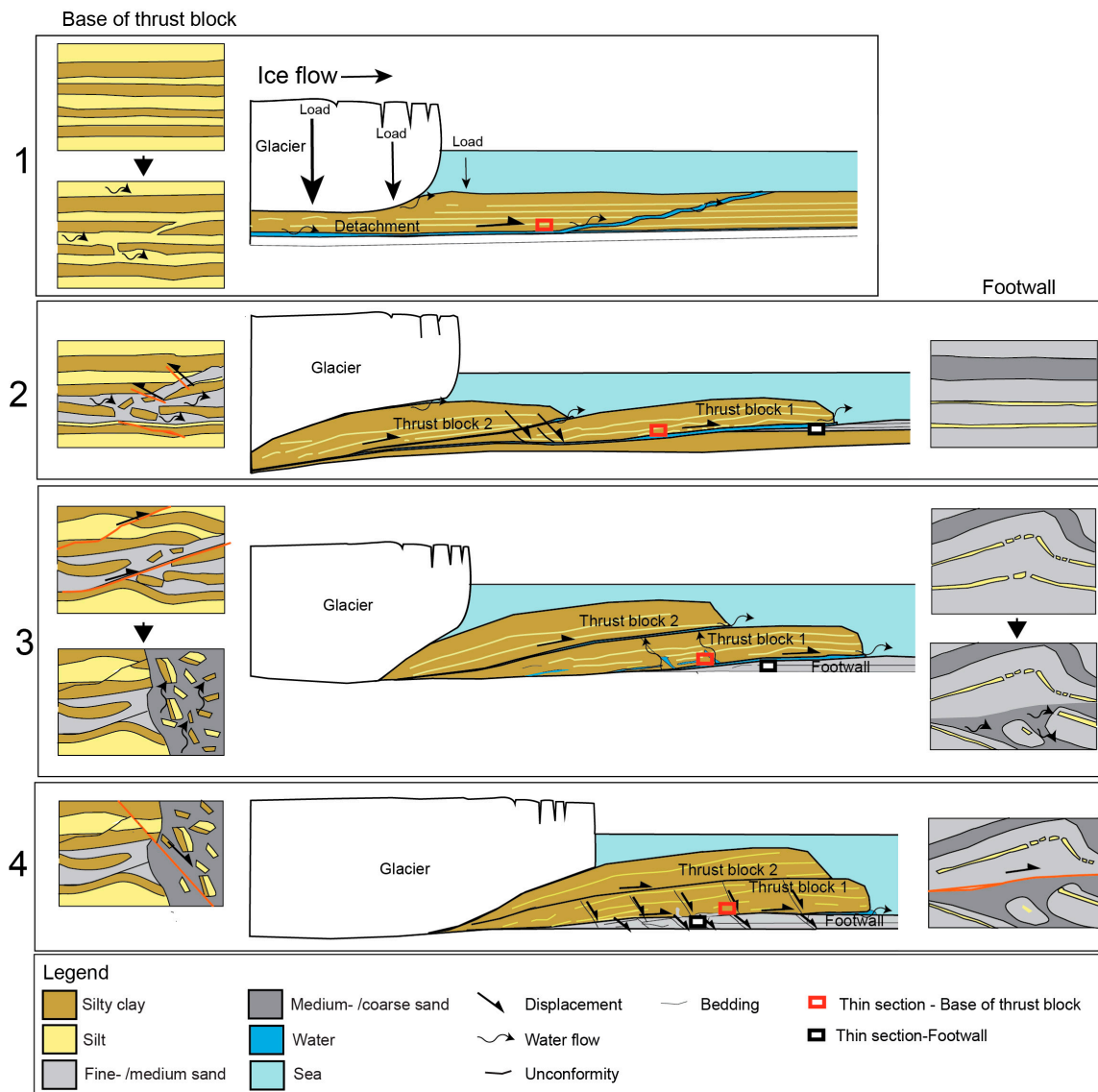
Figure 12. A sequential model explaining micro- and macroscale processes during large-scale glaciectonic thrusting based on investigation of the Melaleiti and Ásgil thrust-block moraines (Paper II). Stage 1: Groundwater pressure rose in response to a glacier advance. This caused liquefaction of the silt and sand, enabling decoupling of sediment blocks. Stage 2: Repeated phases of sediment liquefaction and injection occurred along the detachments. The deformation associated with the transport of the sediment blocks was focused within this relatively thin, water lubricated zone and as a result, they remained largely intact. Stage 3: The leading thrust block was transported on top of permeable sands and gravels in the terminal zone of the glacier. Initially, the thrust block slid over the water-saturated sand and gravel without much internal deformation showing that it was de-coupled from the substratum. However, the frictional drag (and shearing) increased due to water escape towards the margins and possibly increased overburden pressures under the evolving glaciectonic landform. Stage 4: Further draining of the sediments led to brittle deformation (faulting) and lock-up of the thrust-blocks. Figure from Paper II.
