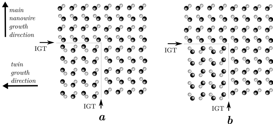
Figure 5.10: Projection models of intergrowth twins (IGTs) in 2H . The twin operation was a 90^\circ rotation around a common (\bar{1}\bar{1}20) axis and the contact plane was \{0001\}/\{\bar{1}\bar{1}00\} , or c -plane / m -plane. Both the growth direction and the polarity was known for the main nanowire, while only the growth direction was only known for the intergrowth twin. A V-polar model in (a) and a III-polar model in (b). There was no obvious way to model a coherent interface between the two crystals, as there was no match between atom types, positions or bonding angles.
