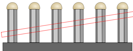
Figure 4.4: Lamella for top-view cross-section of nanowires with an angle relative to the substrate surface. Adjacent nanowires are cut at slightly different positions, progressively from the substrate to the top.
