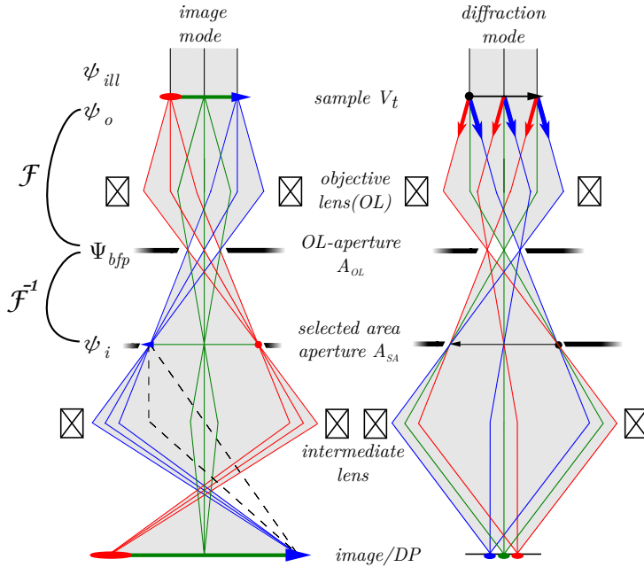
Figure 3.1: Electron wavefunction notation and ray diagrams for the image formation system in both image mode and diffraction mode. The intermediate lens changes the focal length in order to place either the image plane of the objective lens ( \psi_i ) or back focal plane ( \Psi_{bfp} ) in the object plane of the projector lens, which is at the bottom of the illustration. The illumination is parallel and coherent ( \psi_{ill} = 1 ) and the phase in the exit wavefunction ( \psi_o ) depends on the projected sample potential ( V_t ). The color coding in image mode (left) refers to the position on the specimen, while the color coding in diffraction mode (right) refers to the diffraction angle.
