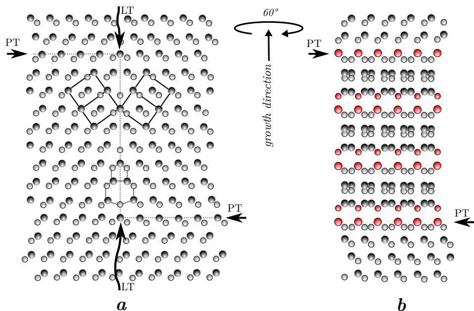
Figure 5.4: Projection models of a lateral twin (LT) in 3C nanowires seen along a \langle 110 \rangle axis with unit cells in black lines. The twin operation was a 60^\circ (or 180^\circ ) rotation around a common \langle 111 \rangle axis, and the contact plane was \{11\bar{2}\} (parallel to the growth direction). (a) Projection through a \langle 110 \rangle zone axis parallel to the contact plane. Every third layer in the growth direction were lined up. (b) Projection through a \langle 110 \rangle zone axis that was 60^\circ from the one in (a) (rotation around the nanowire growth axis). The periodicity along the growth direction was extended by three:
