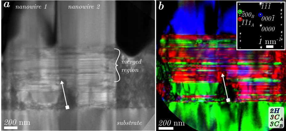
Figure 5.7: Two partially merged 2H GaAs nanowires [III]. BFTEM image (a) and DFTEM images (b) of the substrate, transformed/merged region and the two free-standing nanowires. The arrow indicates where substrate growth hindered the two nanowires from merging. Above the arrow the two merged nanowires shared a perpendicular twinned 3C crystal structure, up to the point where the nanowires no longer touched and exhibited their original 2H structure. The inset shows a SAED ( 2H [\bar{1}\bar{1}20] , 3C_A [\bar{1}10] and 3C_B [01\bar{1}] ) pattern recorded from the area in (b) with a corresponding color coding. Note that the forbidden 0001 spot is available here due to double diffraction.
