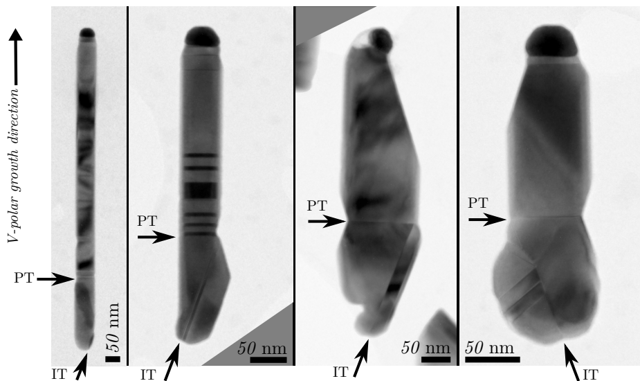
Figure 5.3: Inclined (IT) and perpendicular twins (PT) in InAs nanowires synthesised without crystalline support [II]. All nanowires have been determined to grow in the V-polar \langle \bar{1}\bar{1}\bar{1} \rangle direction using convergent beam electron diffraction.
