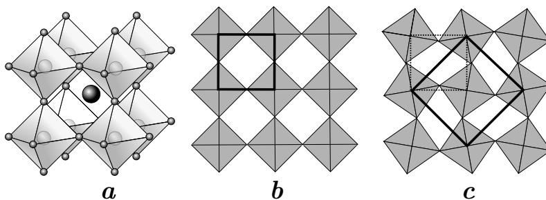
Figure 2.2: (a) Coordination polyhedra model of perovskite ( ABO_3 ). The large dark sphere is A, the small spheres are O and the spheres inside the octahedra are B. (b) Side view projection of the network of corner-sharing octahedra in the cubic structure. (c) The network of corner-sharing octahedra in a tetragonal structure where the octahedra are tilted. The unit cells are outlined by solid lines.
