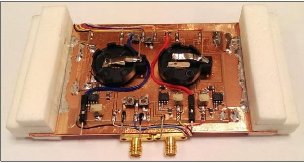
Fig. 4. Prototype B – prototype with integrated tuners (bottom view).
