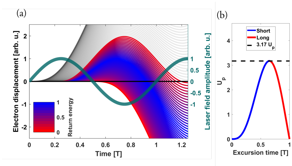
Figure 2.4: (a) Classically calculated electron trajectories as a function of laser period T . The trajectories are released during the first half of the driving field laser cycle 0 < T < 0.5 . The trajectories are color coded to display return energy for each tunneling time. Grey trajectories never return to the parent ion. (b) Return energy of the different trajectories as a function of their excursion times, showing two classes of trajectories leading to the same energy. The highest energy is 3.17 U_p , where U_p is the ponderomotive energy.
