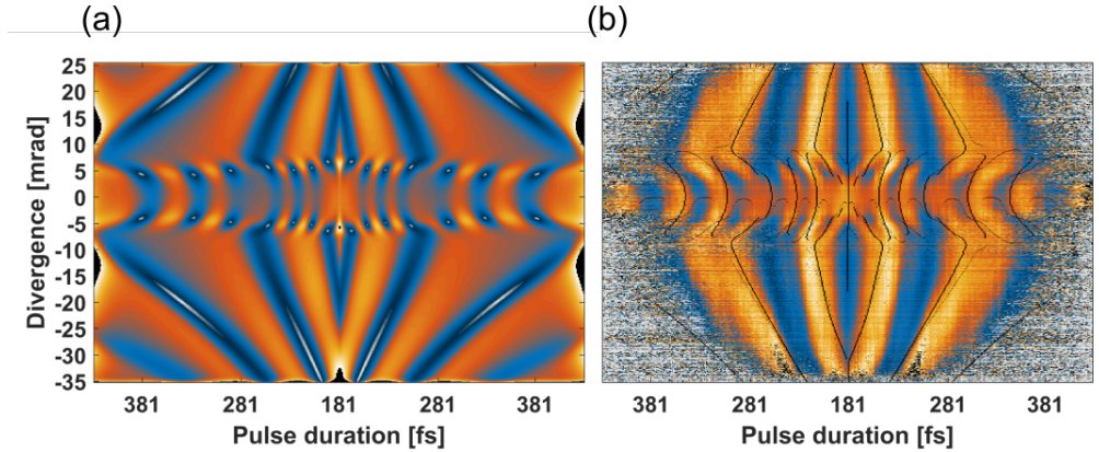
Figure 3.II: (a) Optimized result from the Gaussian beam model for harmonic 15 in argon. The crests from the interference fringes from the theoretical model are overlaid on the measured chirp-scan (b)
