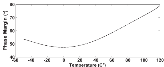
Fig. 6. OTA phase margin versus temperature with enhanced phase compensation.
