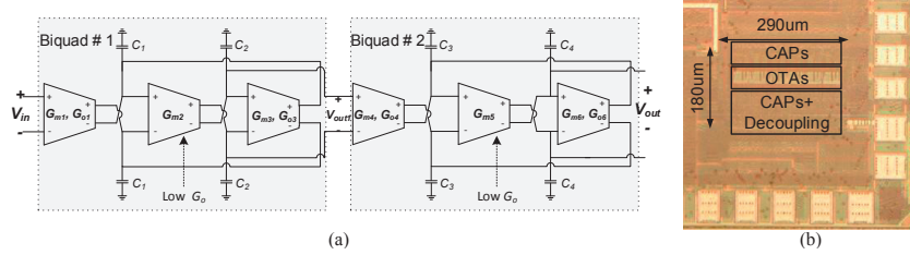
Fig. 4. (a) Schematic of the fourth order OTA-C filter and (b) die micrograph.
