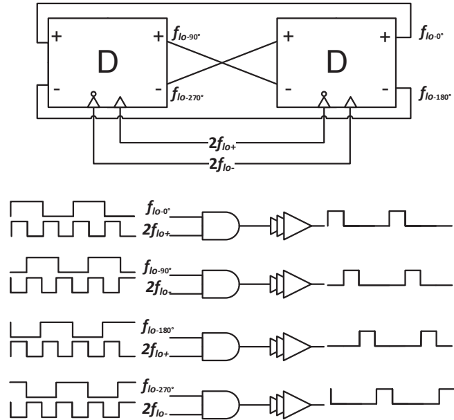
Figure 3.8: LO generation of quadrature signals with 25% duty cycle.
