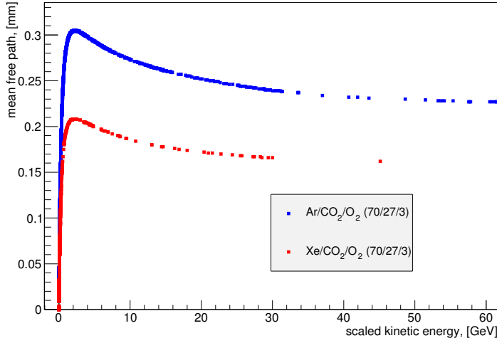
Figure 3.11.: Mean free path of a relativistic muon as a function of scaled kinetic energy \left(E_{kin} \frac{m_{proton}}{m_{particle}}\right) for Xenon- and Argon-based gas mixtures.
