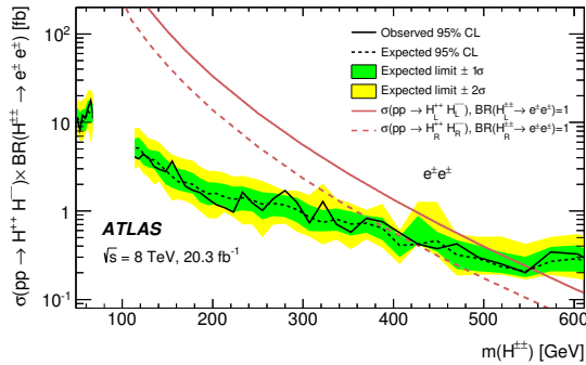
Figure 5.20.: Upper limits at 95% C.L. on the cross section as a function of e^{\pm} e^{\pm} invariant mass for the production of a doubly charged Higgs boson assuming a 100% branching ratio to e^{\pm} e^{\pm} . The green and yellow bands correspond to the 1\sigma and 2\sigma bands on the expected limits respectively. Pair production cross sections for left and right-handed H^{\pm\pm} are overlaid.
