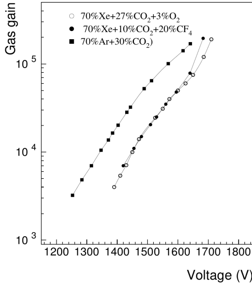
Figure 3.4.: Straw gas gain as a function of high voltage for different gas mixtures [27].
