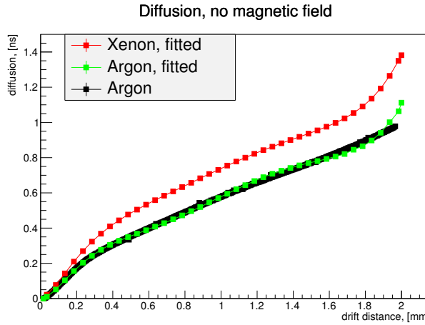
Figure 3.14.: Electron drift-diffusion in Xenon- (red) and Argon-based (green) gas mixtures as modelled in the digitization package (with a 4-th degree polynomial). Black points correspond to the Garfield simulation for the an Argon-based gas mixture.
