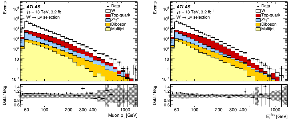
Figure 6.16.: Muon p_T (left) and E_T^{\text{miss}} (right) distributions after the final selection. The uncertainty band in the ratio plot indicate the sum in quadrature of the systematic uncertainties.
