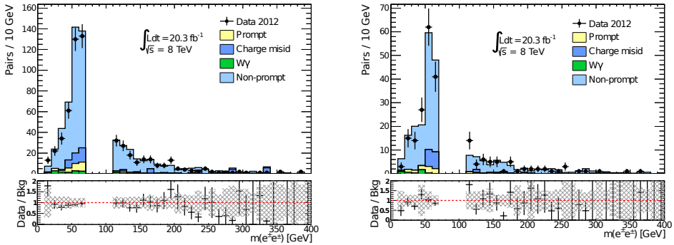
Figure 5.12.: Invariant e^{\pm}e^{\pm} mass distribution plots of prediction and data in the VR with subleading electron passing weaker isolation (left) and in the VR with leading electron passing weaker isolation (right). The hatched areas show the statistical uncertainty of the background prediction.
