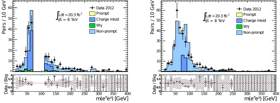
Figure 5.11.: Invariant e^{\pm}e^{\pm} mass distribution plots of prediction and data in the VR with both electron passing medium electron identification criteria (left) and in the VR passing weaker isolation (right). The hatched areas show the statistical uncertainty of the background prediction.
