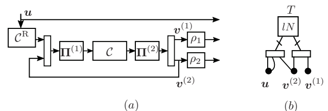
Fig. 2. A unified ensemble based on a single trellis (a) encoder block diagram (b) compact graph.
